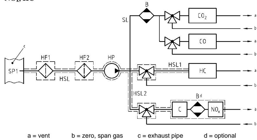
Figure 9 Schematic flow diagram of raw exhaust gas analysis system for CO, CO 2 , NO x , HC
