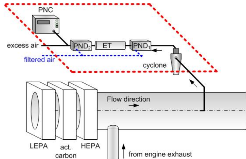
Figure 4.20 Schematic of Recommended Particle Sampling System – Full Flow Sampling
