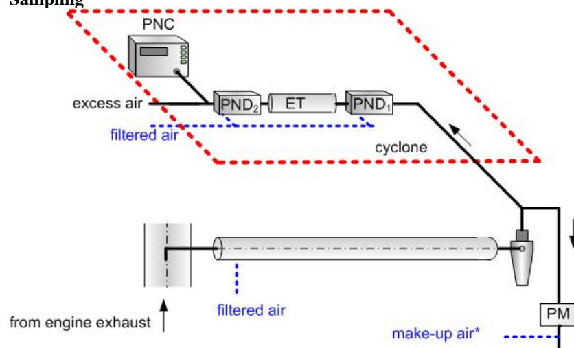
Figure 1419 Schematic of Recommended Particle Sampling System – Partial Flow Sampling
