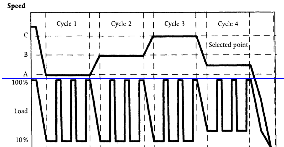
Figure 3 Sequence of ELR Test
