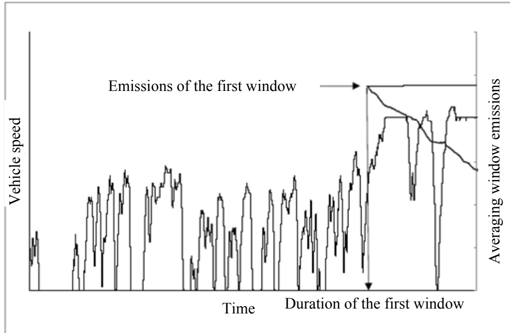
Figure 1. Vehicle speed versus time and Vehicle averaged emissions, starting from the first averaging window, versus time.
