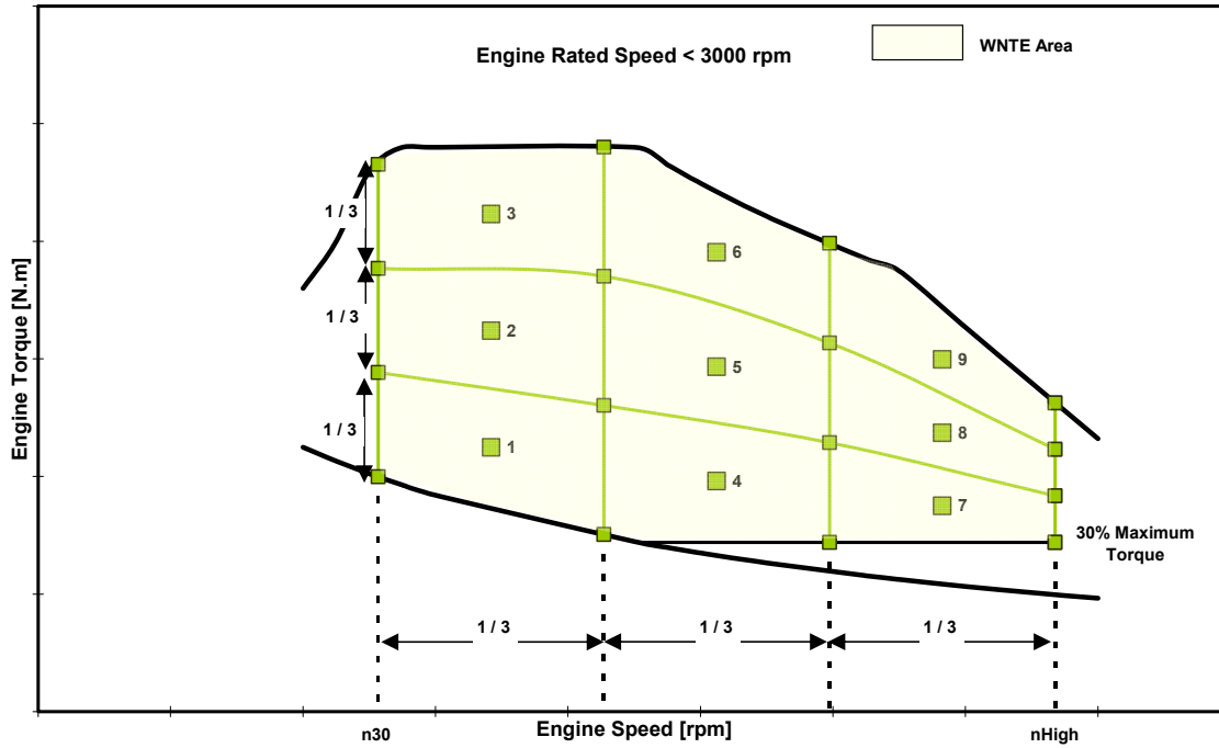
Figures 5 and 6 WNET test cycle grids
