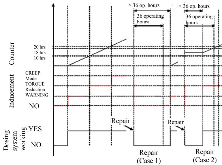
Figure 4 Failure of the reagent dosing system
