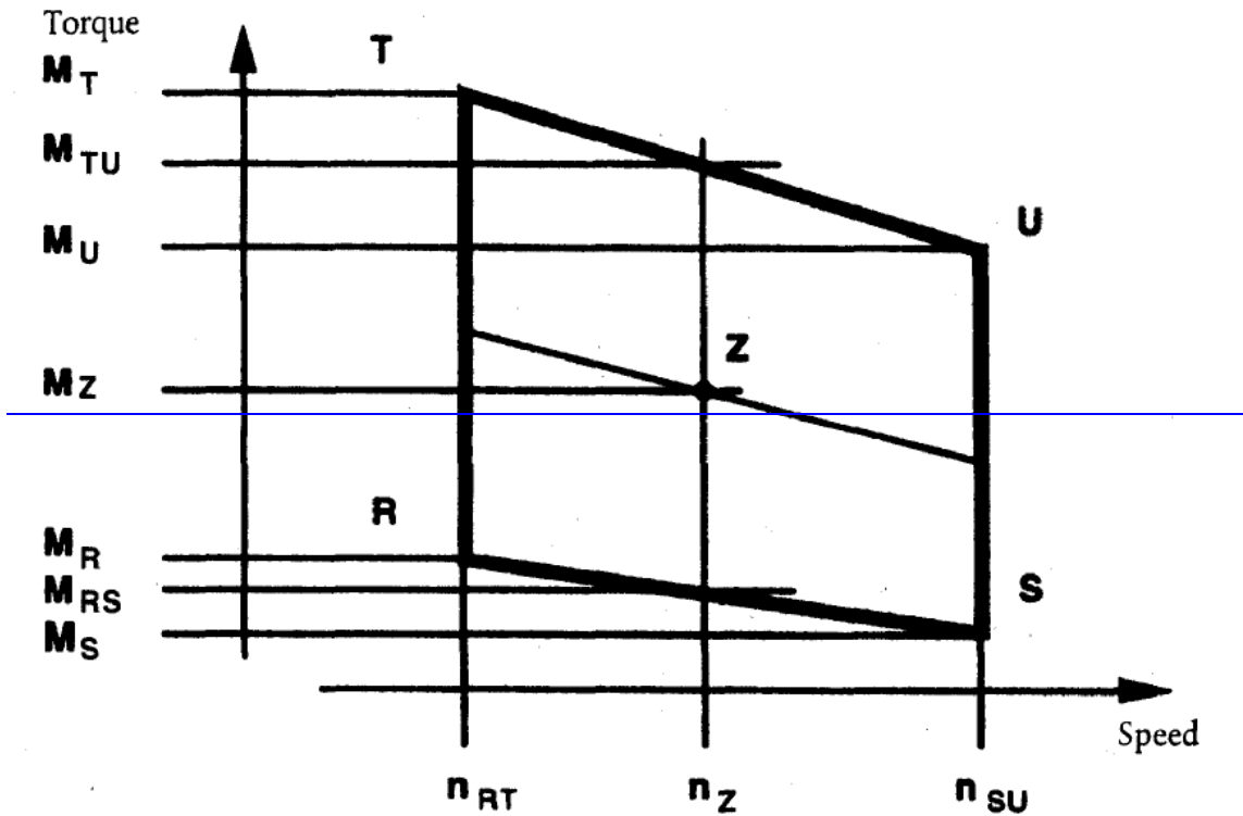
Figure 4 Interpolation of NO x Control Point
