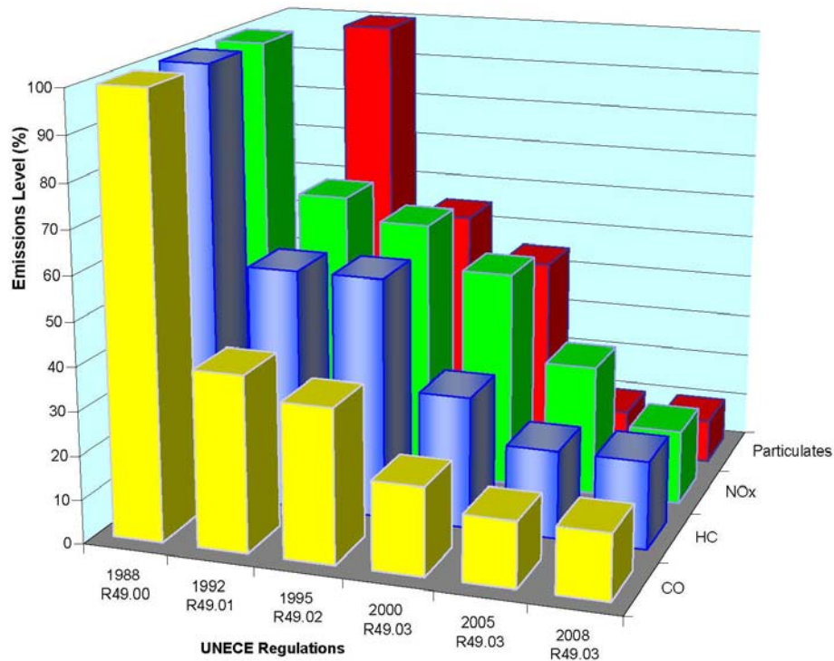
Figure 3 Evolution of emission limits of heavy duty vehicles
