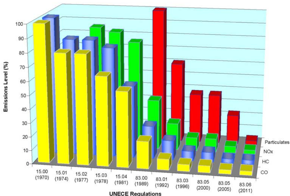
Figure 2 Evolution of emission limits of passenger cars
