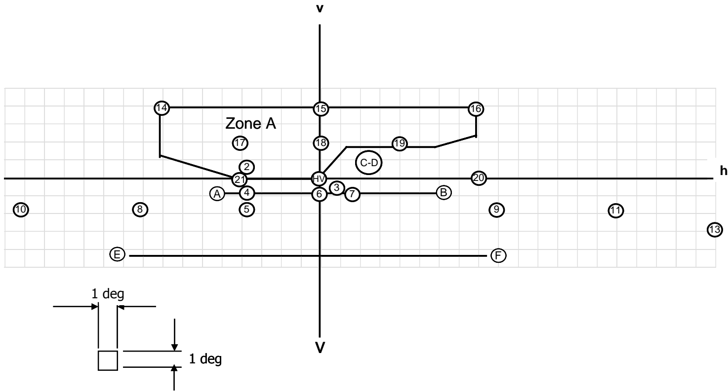
Figure B: Passing beam for right-hand traffic
