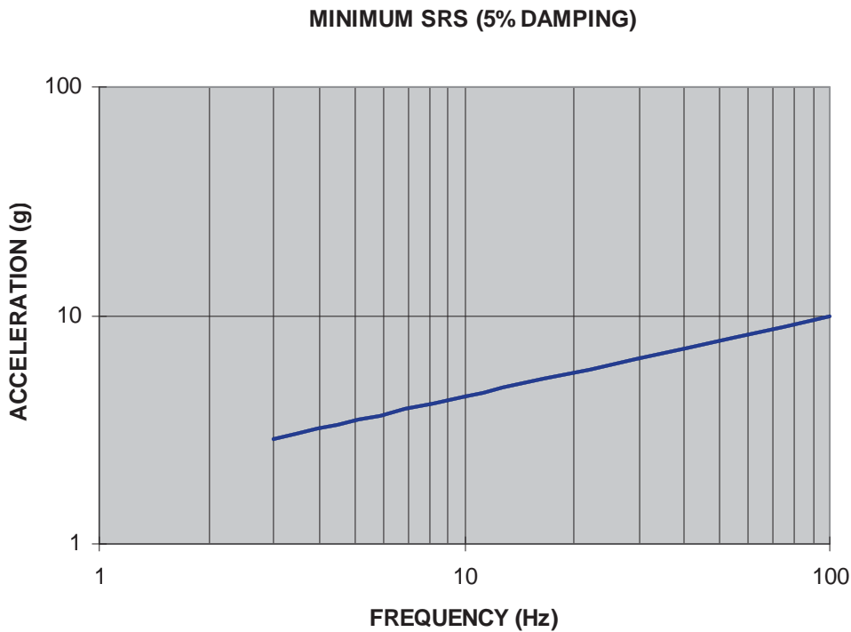
Figure 41.3.8.1: Minimum SRS Curve
