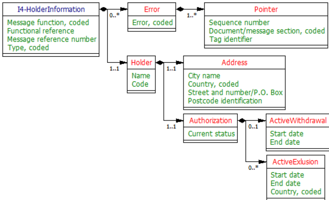
Holder information UML diagram
