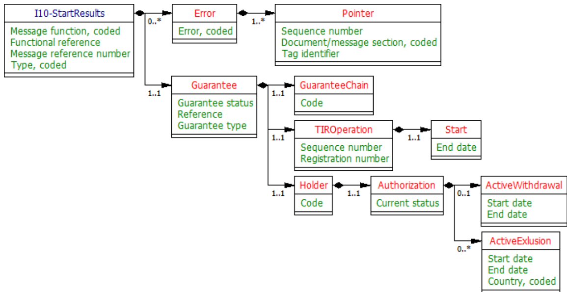
Start results UML diagram
