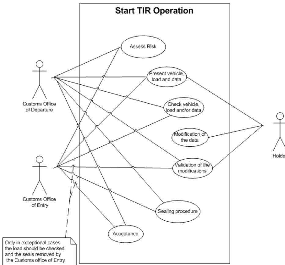
Figure 1.16 Start TIR operation use case diagram
