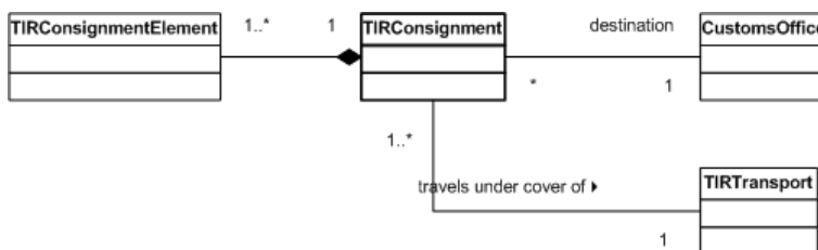
Figure 1.25 TIR consignment class and its relationships
