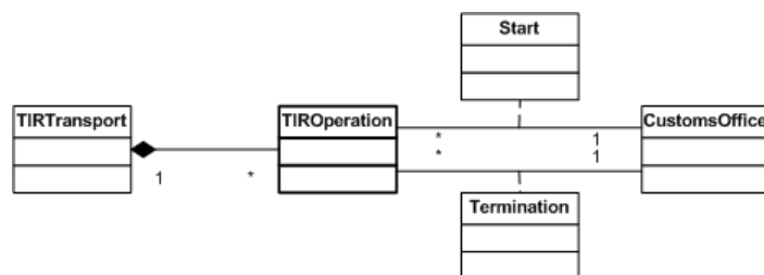
Figure 1.24 TIR operation class and its relationships
