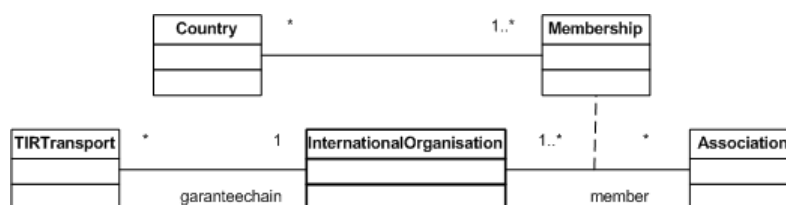
Figure 1.19 International organization class and its relationships
