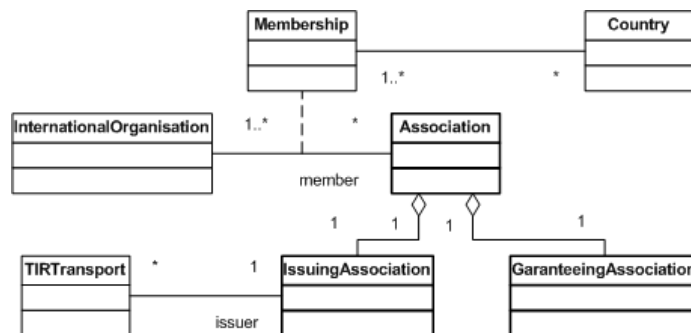
Figure 1.20 Association class and its relationships
