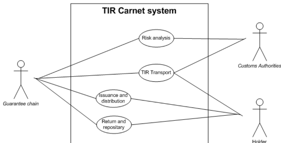
Figure 1.7 TIR Carnet system use case diagram
