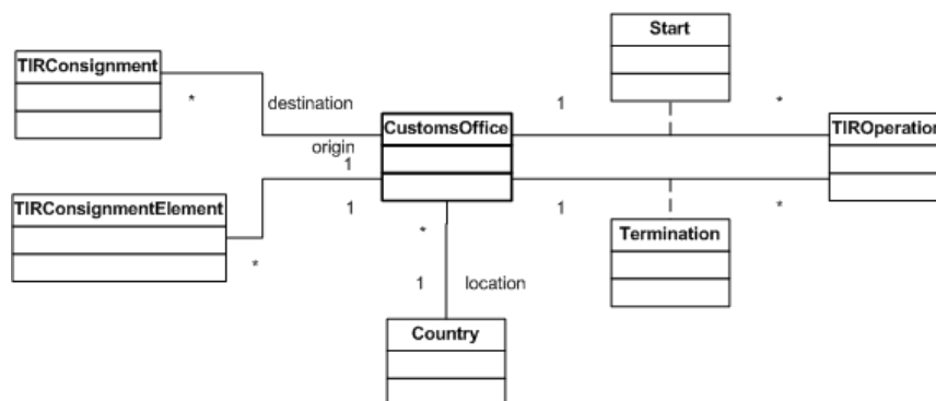
Figure 1.28 Customs office class and its relationships
