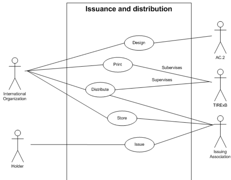
Figure 1.9 Issuance and distribution use case diagram
