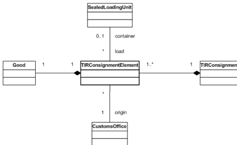
Figure 1.26 TIR consignment element class and its relationships
