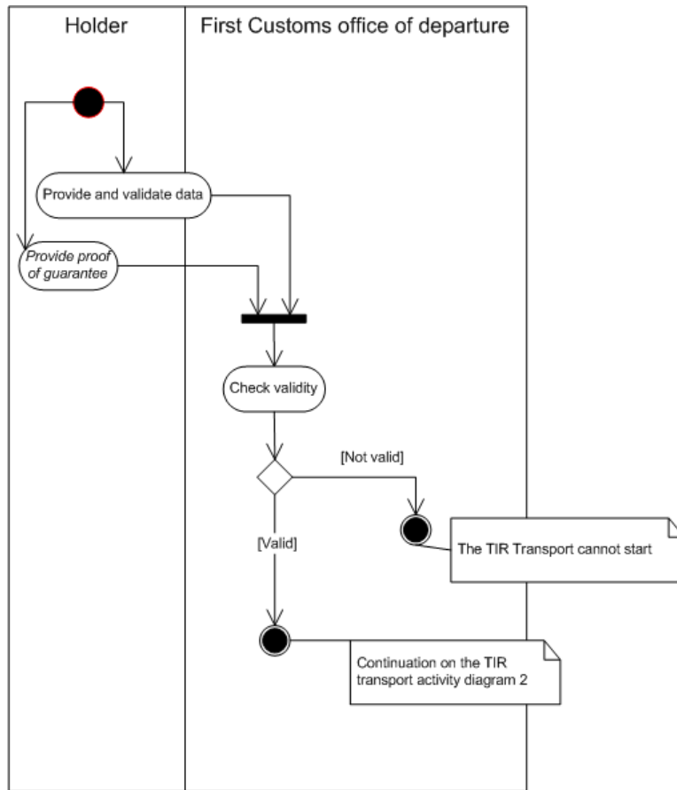
Figure 1.12 TIR transport activity diagram 1
