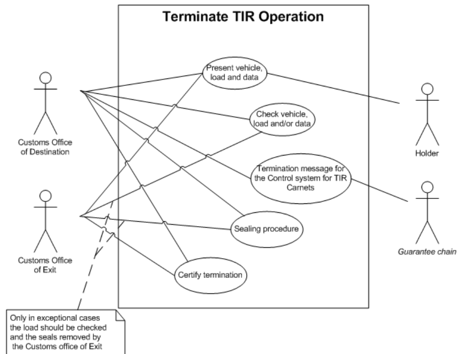
Figure 1.17 Terminate TIR operation use case diagram
