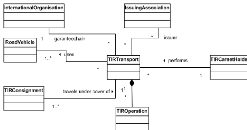
Figure 1.23 TIR transport class and its relationships
