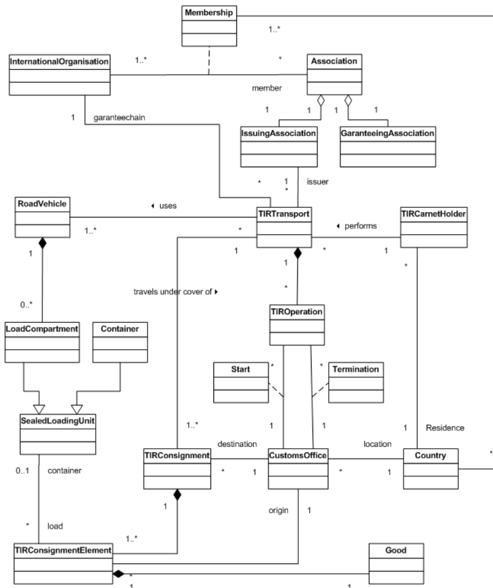
Figure 1.18 High level class diagram
