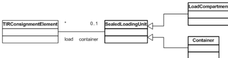
Figure 1.22 Sealed loading unit class and its relationships
