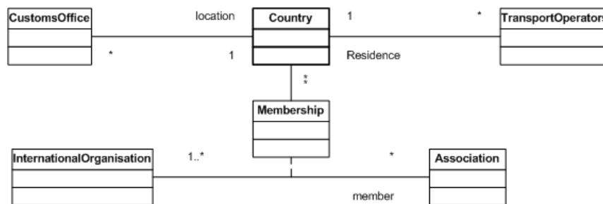
Figure 1.29 Country class and its relationships
