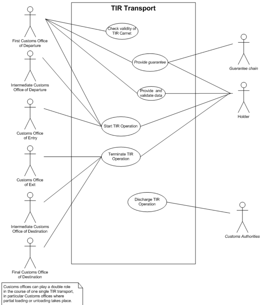
Figure 1.11 TIR transport use case diagram
