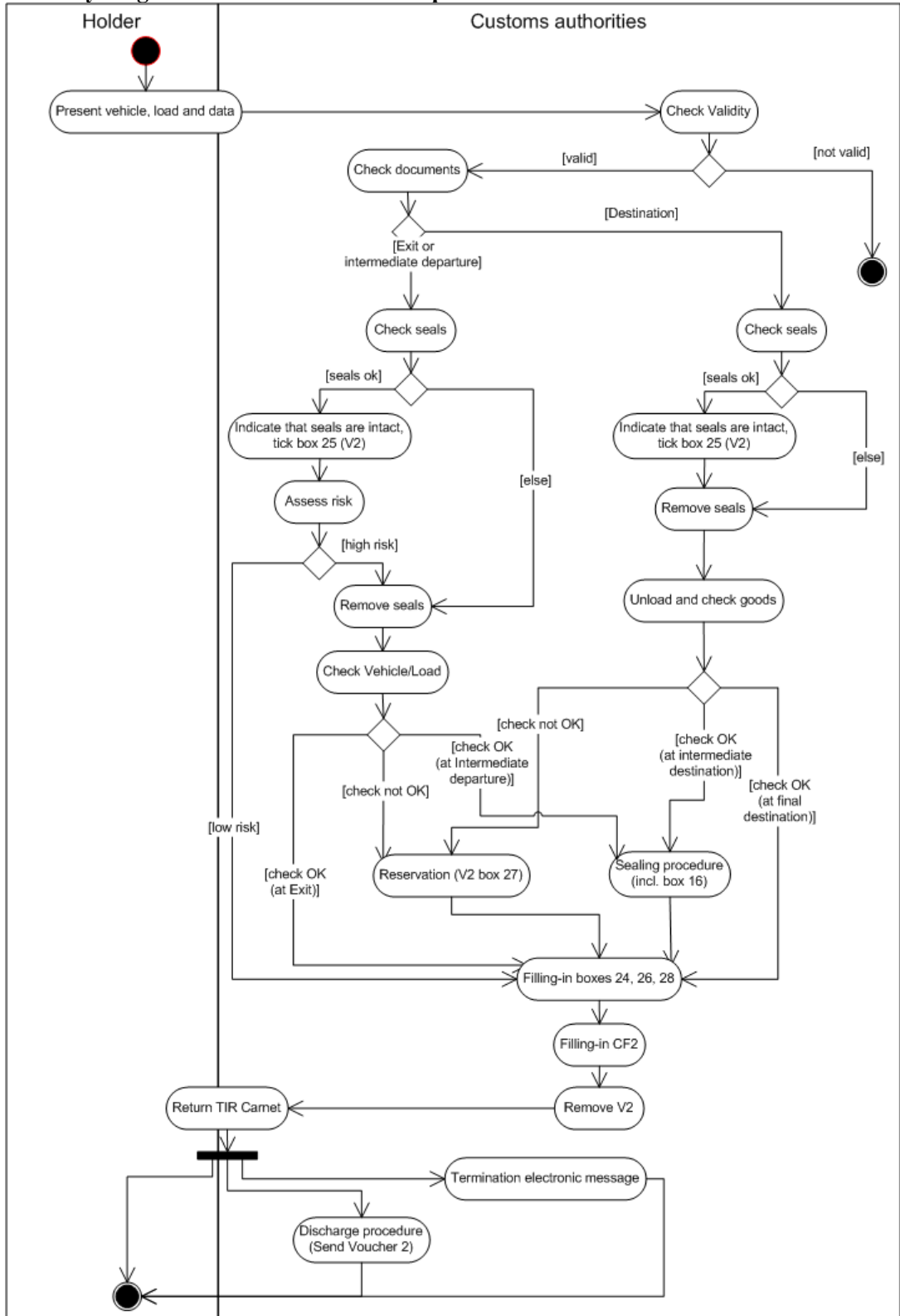
Figure 1.16 Terminate TIR operation activity diagram
