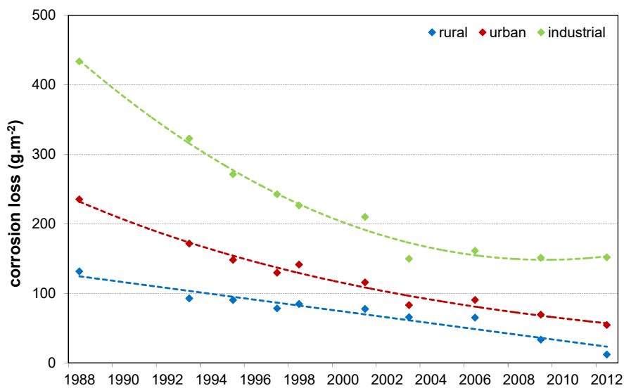
Figure 22: Trends in carbon steel yearly corrosion loss based on results from 20 test sites.
