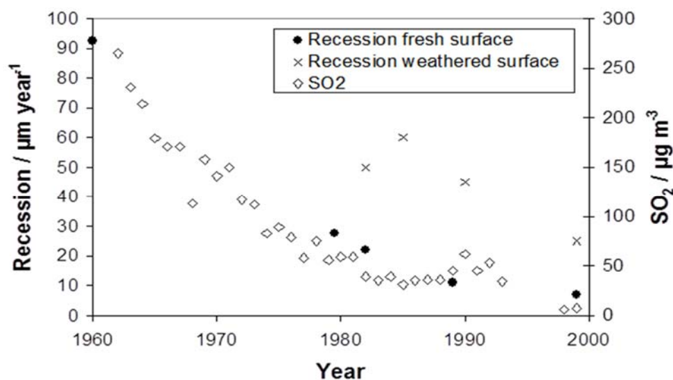
Figure 23: Surface recession rates of limestone and \text{SO}_2 concentration at St Paul's Cathedral. The surface recession of fresh surfaces is measured on standard samples while recession on weathered surfaces is measured on the actual building using micro-erosion meters.
