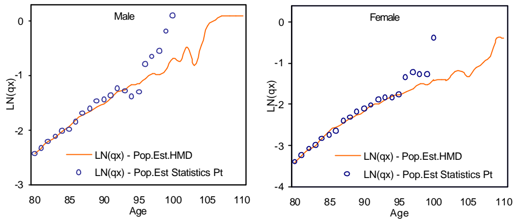
Figure 4 – Mortality rates for the oldest-old
