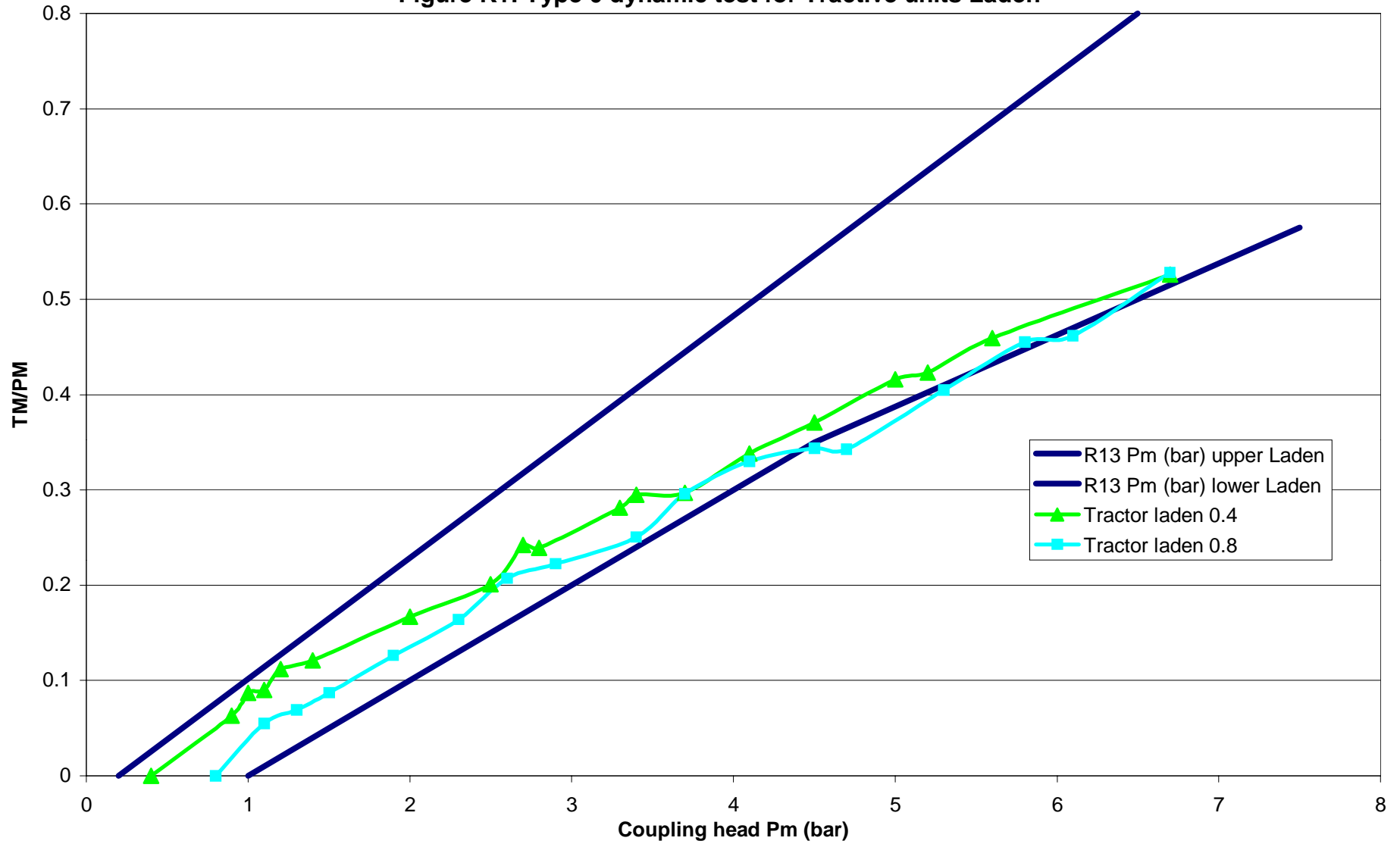
Figure K1: Type 0 dynamic test for Tractive units Laden
