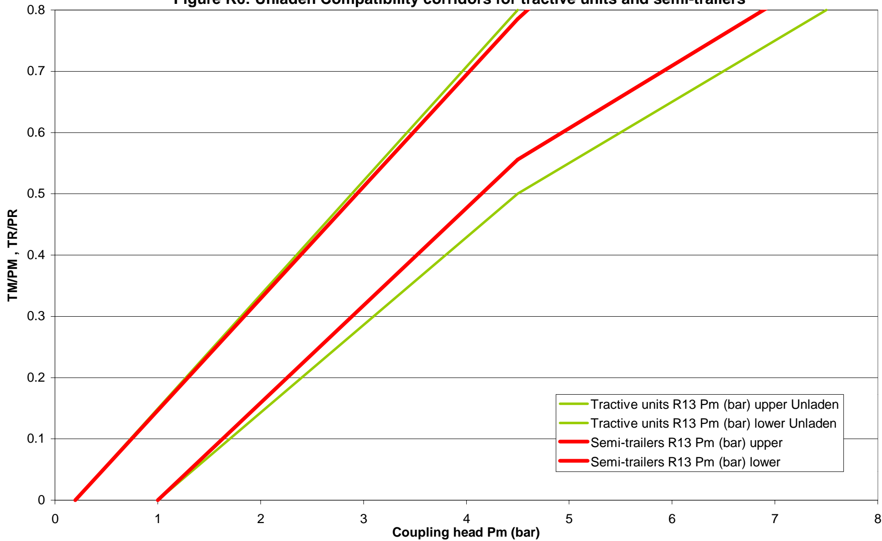
Figure K6: Unladen Compatibility corridors for tractive units and semi-trailers
