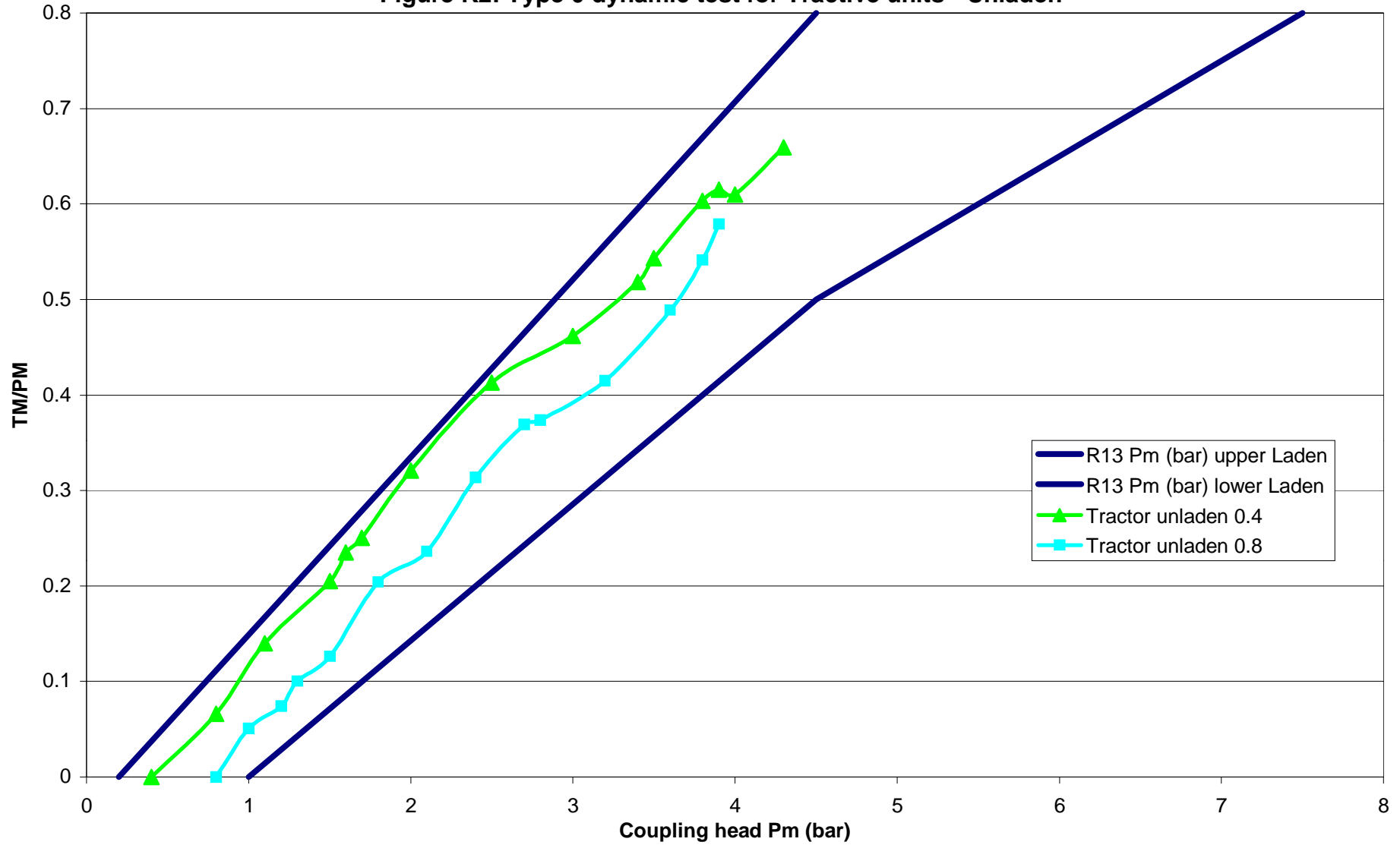
Figure K2: Type 0 dynamic test for Tractive units - Unladen
