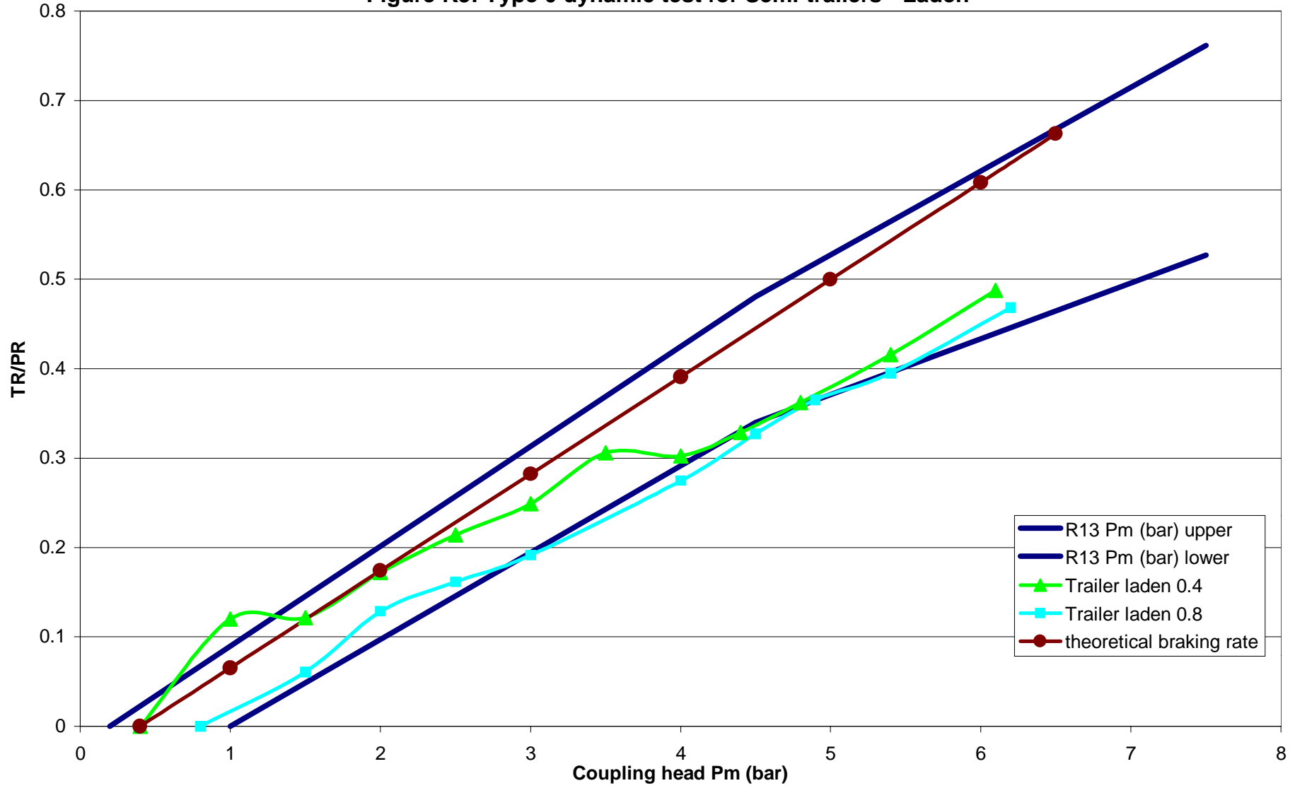
Figure K3: Type 0 dynamic test for Semi-trailers - Laden
