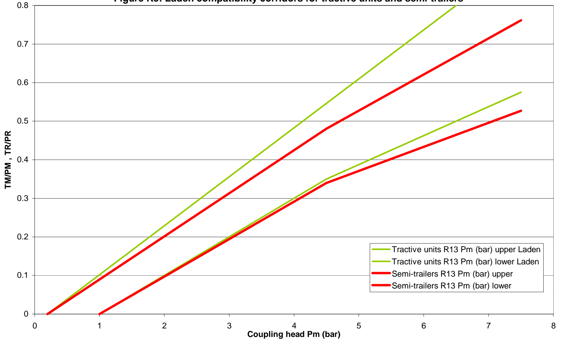
Figure K5: Laden compatibility corridors for tractive units and semi-trailers
