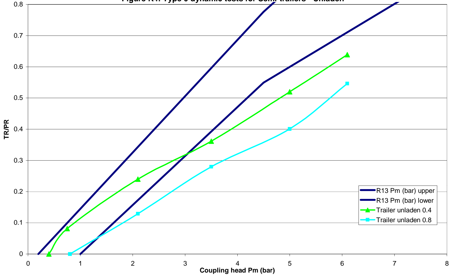
Figure K4: Type 0 dynamic tests for Semi-trailers - Unladen
