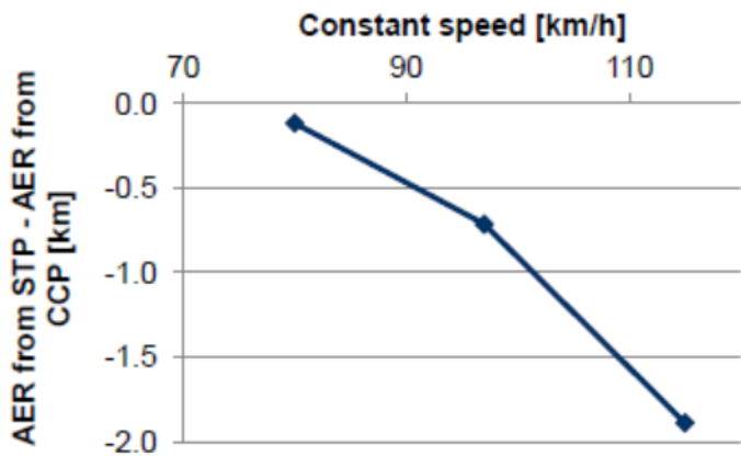
Figure 26 Validation data for shortened test procedure provided by ACEA (BMW)
