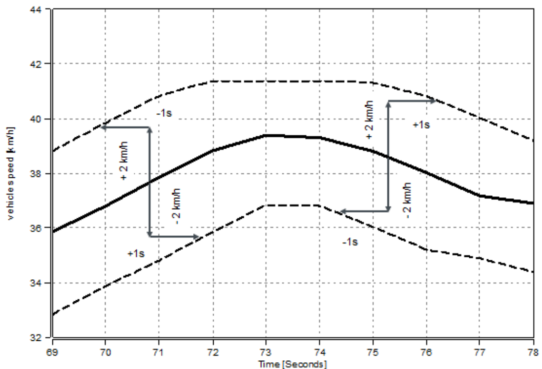
Speed trace tolerances
