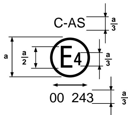
a \geq 5 mm for Class A headlamp
