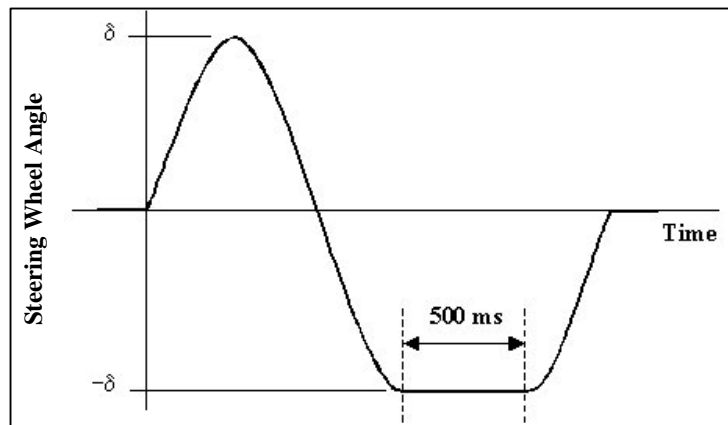
Figure 2 Sine with Dwell
