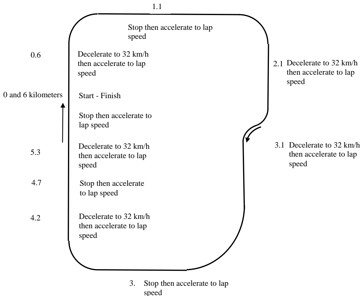
Figure A9/1 Driving schedule
