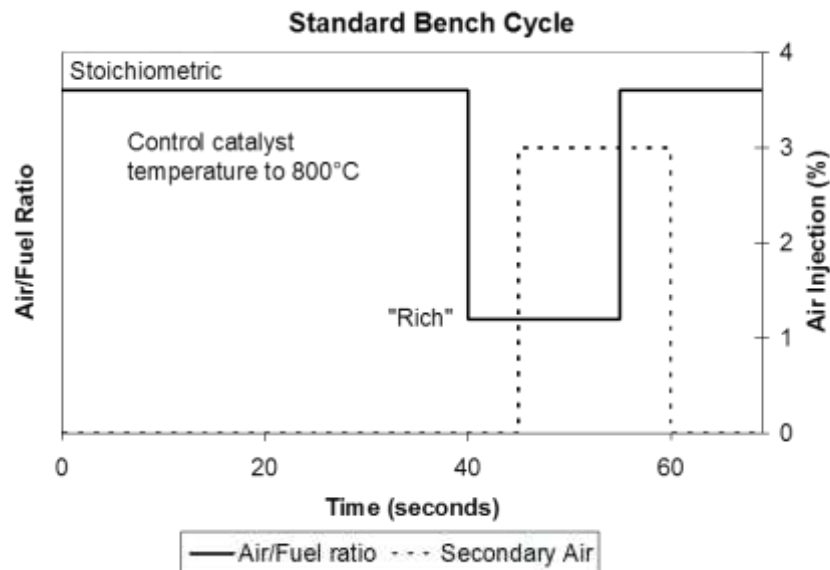
Figure A9.App1/2 Standard Bench Cycle
