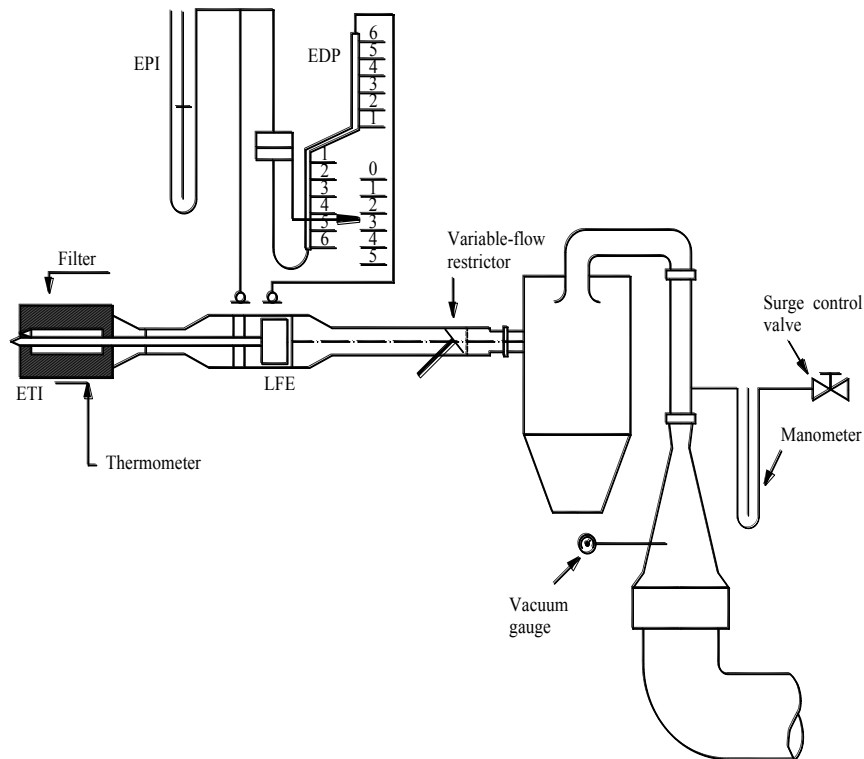
Figure A4a.App2/9 CFV calibration configuration
