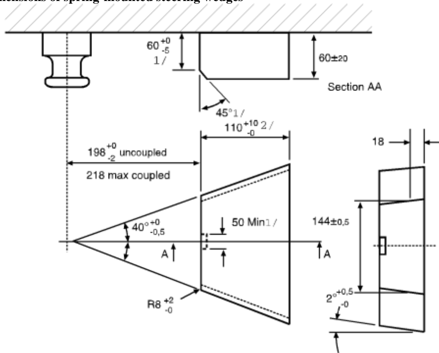
Figure 17 Dimensions of spring-mounted steering wedges
