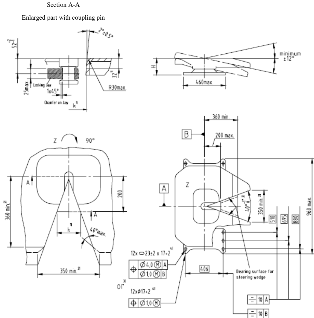
Figure 16 Dimensions of standard fifth wheel couplings (see Table 11)
