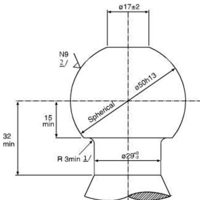
Figure 2 Coupling ball of Class A
