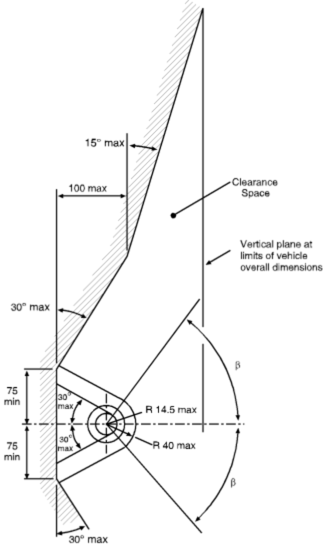
Figure 25b Clearance space for coupling ball - plan view
