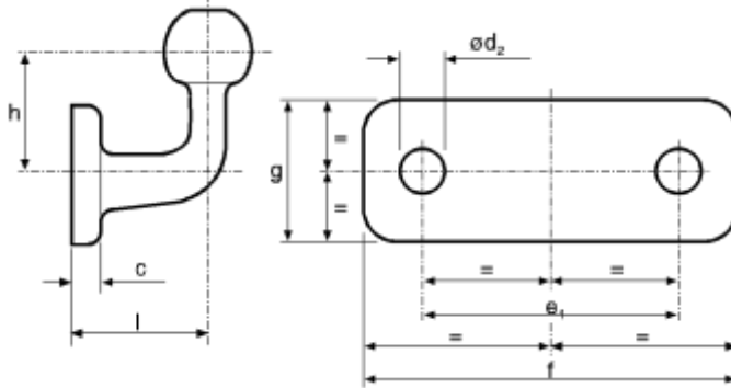
Figure 4 Dimensions of standard flange type ball couplings of Class A50-2 to A50-5 (see Table 2)
