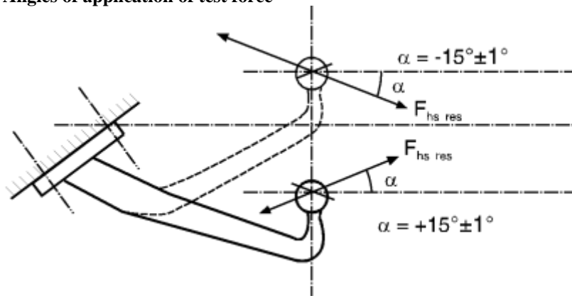
Figure 21 Angles of application of test force
