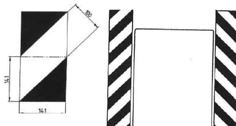
"Figure 1 Retro-reflective material marking of Class F
