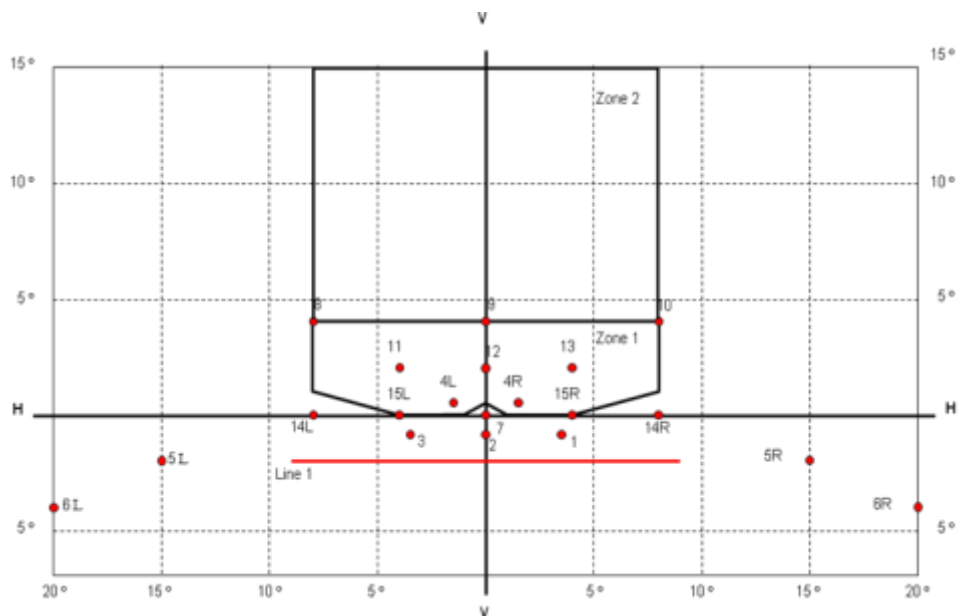
Figure D Passing beam - position of test points and zones for Classes C, D and E headlamp(s):
