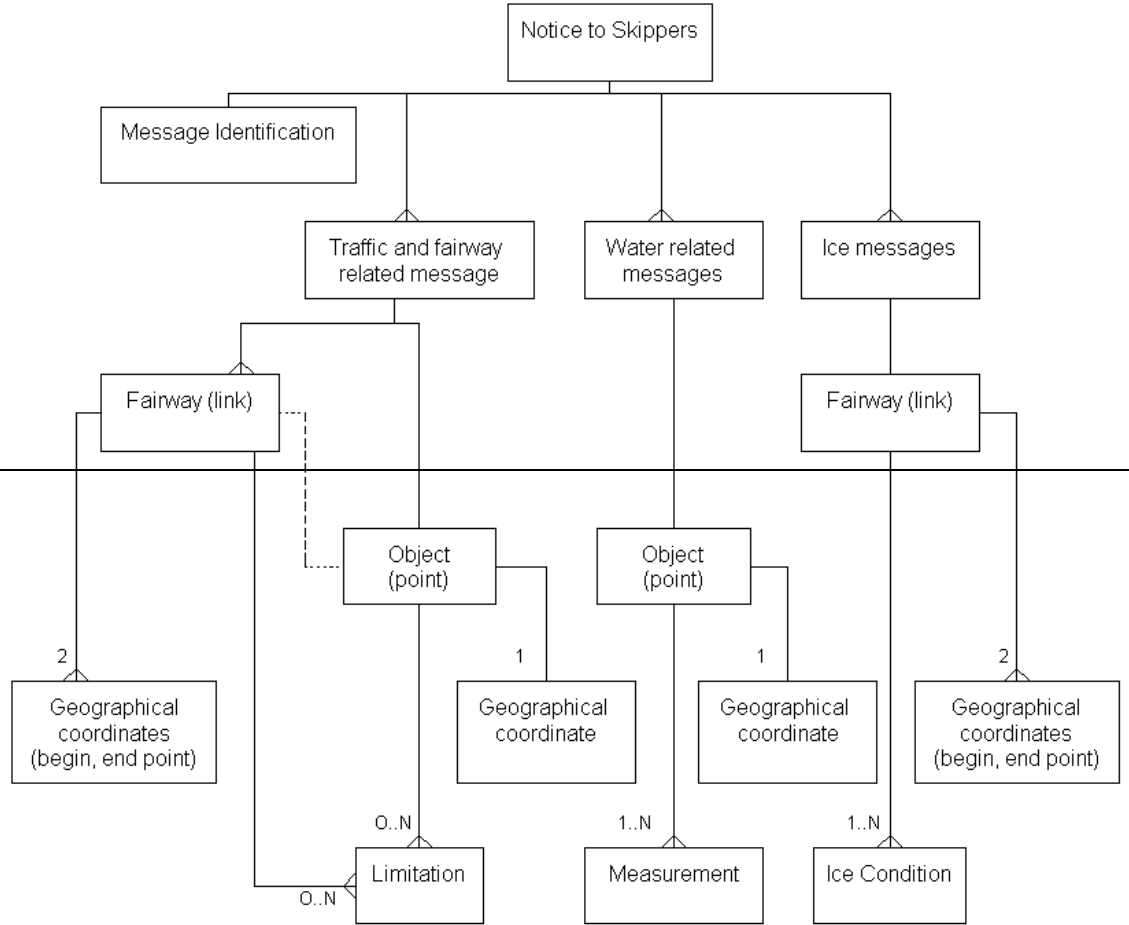
Figure 7.1.2 Notice to Skippers Message structure
