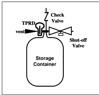
Figure 1 Typical compressed hydrogen storage system
