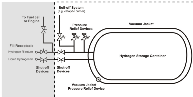
Figure 4 Typical liquefied storage system
