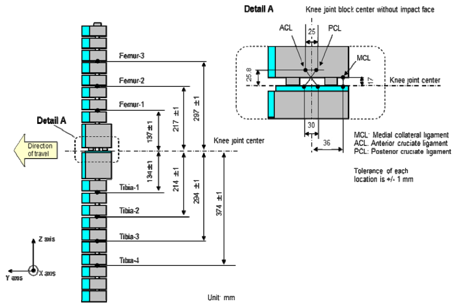
Figure 16 Flexible lower legform impactor; Instrument
