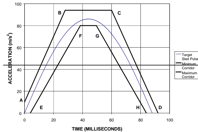
Figure 9-1 Sled pulse acceleration corridor.
