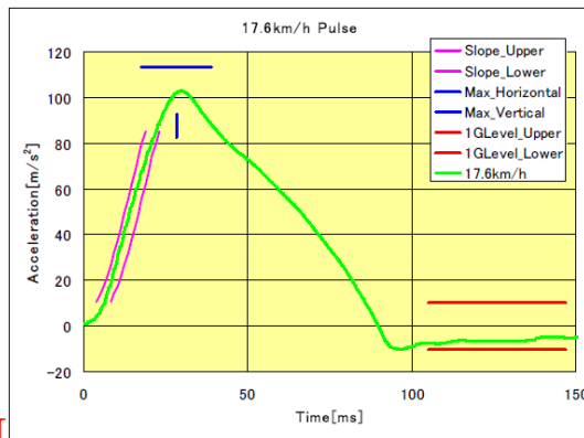
Figure 9-3 Impact Waveform and Permissible Range of Waveform
