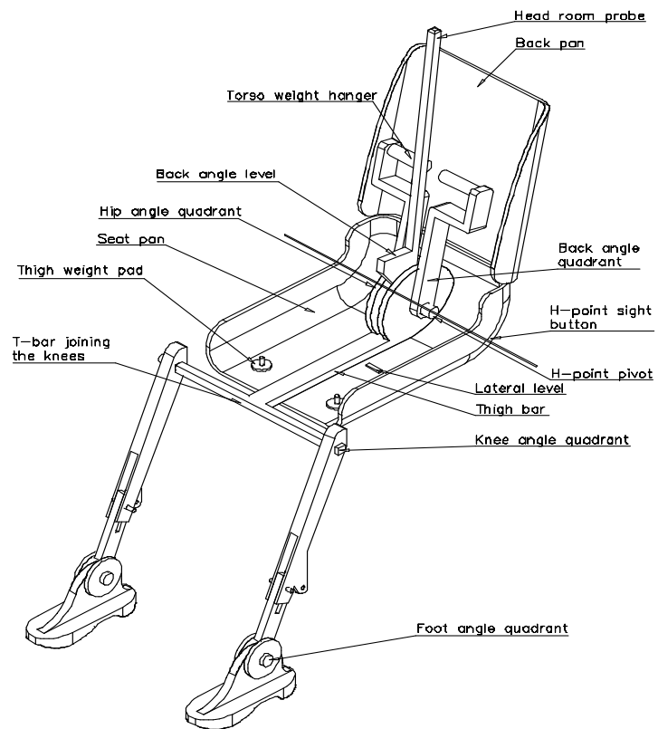
[Figure 11-1 - 3-D H machine elements designation]
