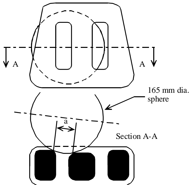
Figure 3-1 - Measurement of a vertical gap "a".
