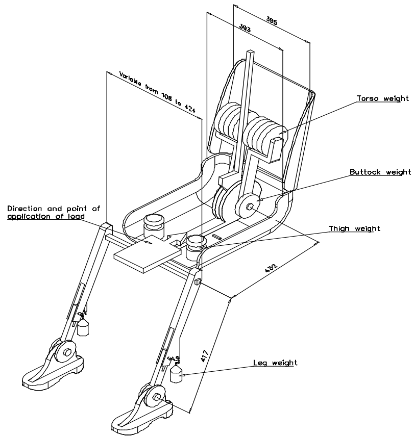
[Figure 11-2 - Dimensions of the 3-D H machine elements and load distribution (Dimensions in millimeters)]
