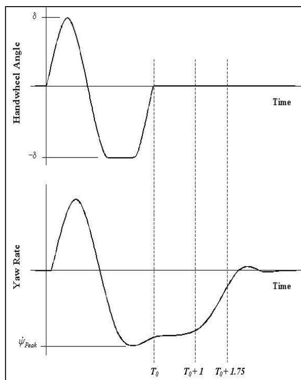
Figure 1 Steering wheel position and yaw velocity information used to assess lateral stability.
