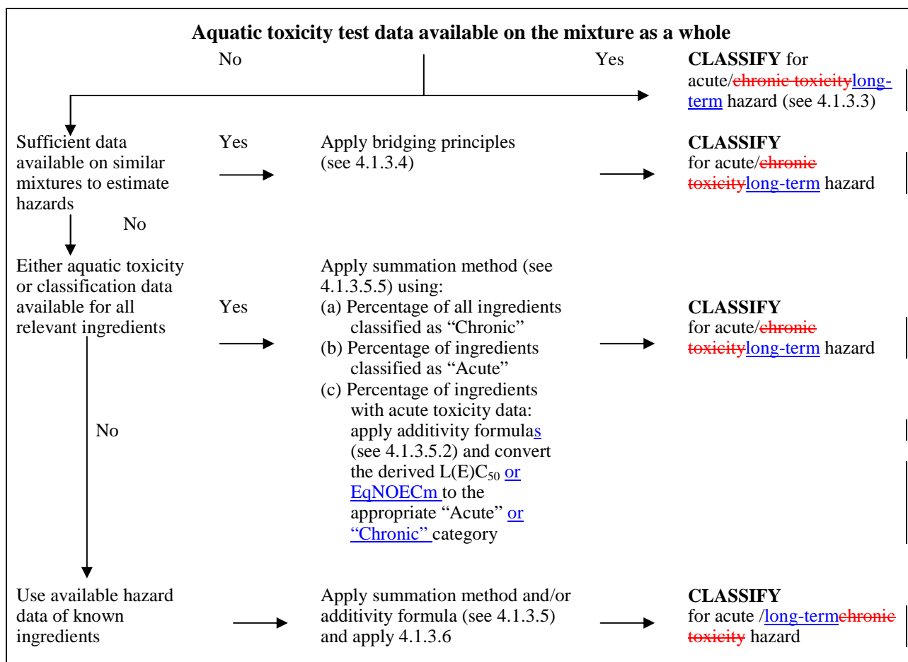
Figure 4.1.2: Tiered approach to classification of mixtures for acute and chronic long-term aquatic environmental hazards
