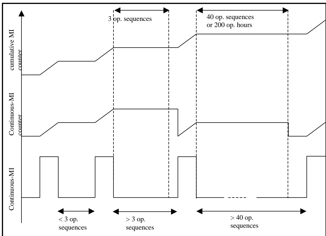
Figure C2: Illustration of the B1 counter activation principles
