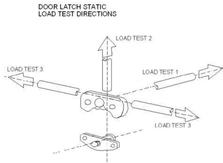
Figure 1-4 – Door Static
