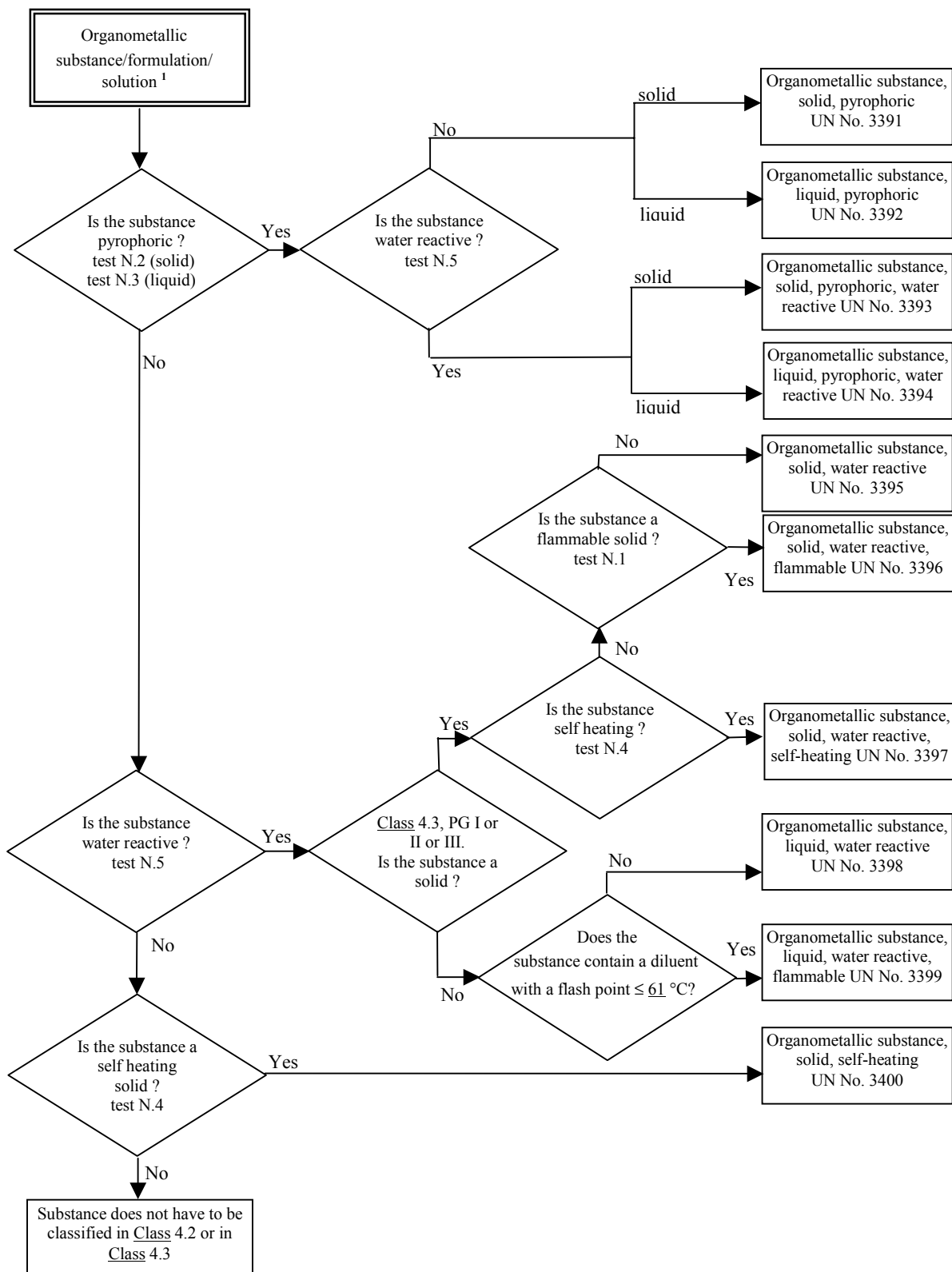
Figure 2.4.2 2.1.5: Flowchart scheme for organometallic substances 2
