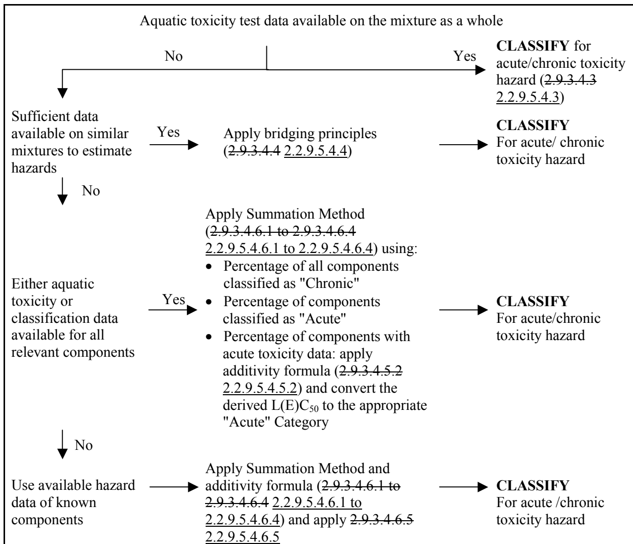
Figure 2.9.1 2.2.9.5.4.2: Tiered approach to classification of mixtures for acute and chronic aquatic environmental hazards
