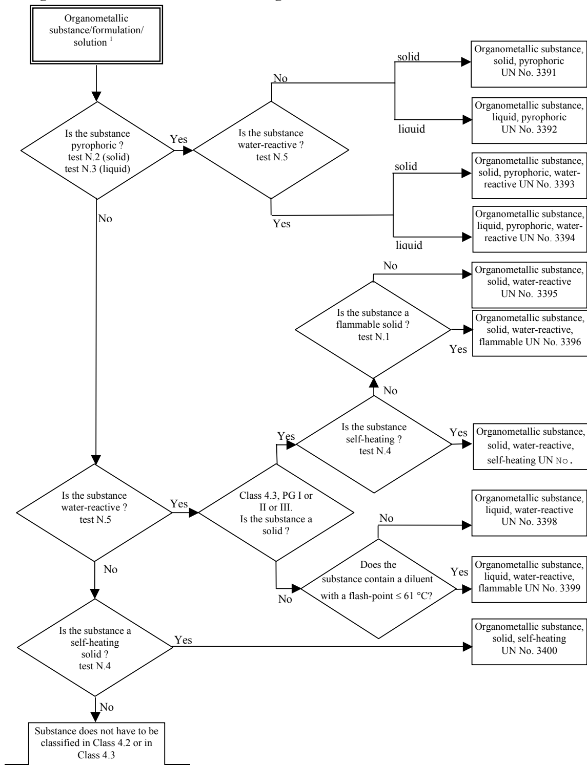
Figure 2.3.6: Flowchart scheme for organometallic substances in Classes 4.2 and 4.3 2
