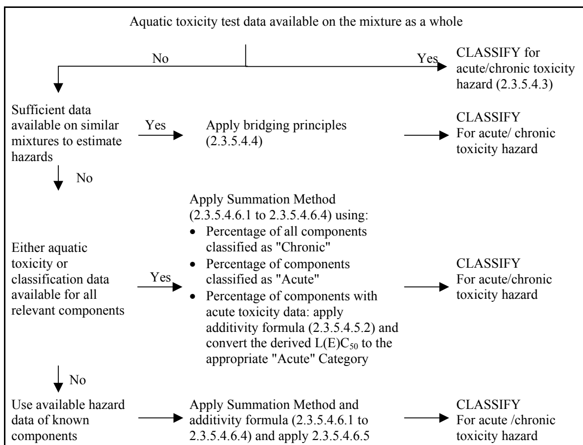
Figure 2.3.5.4.2: Tiered approach to classification of mixtures for acute and chronic aquatic environmental hazards
