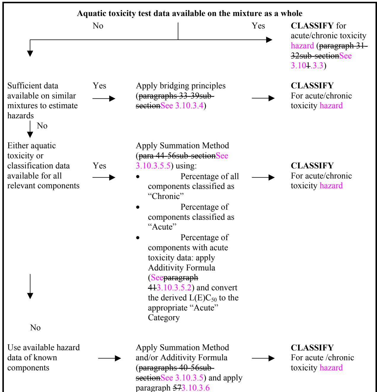
Figure 3.10.2: Tiered approach to classification of mixtures for acute and chronic aquatic environmental hazards
