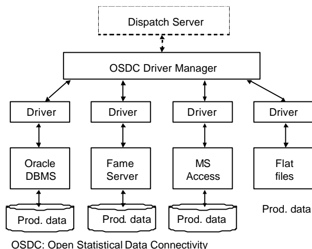
Figure 4. Database federation mechanism in the Storage System
