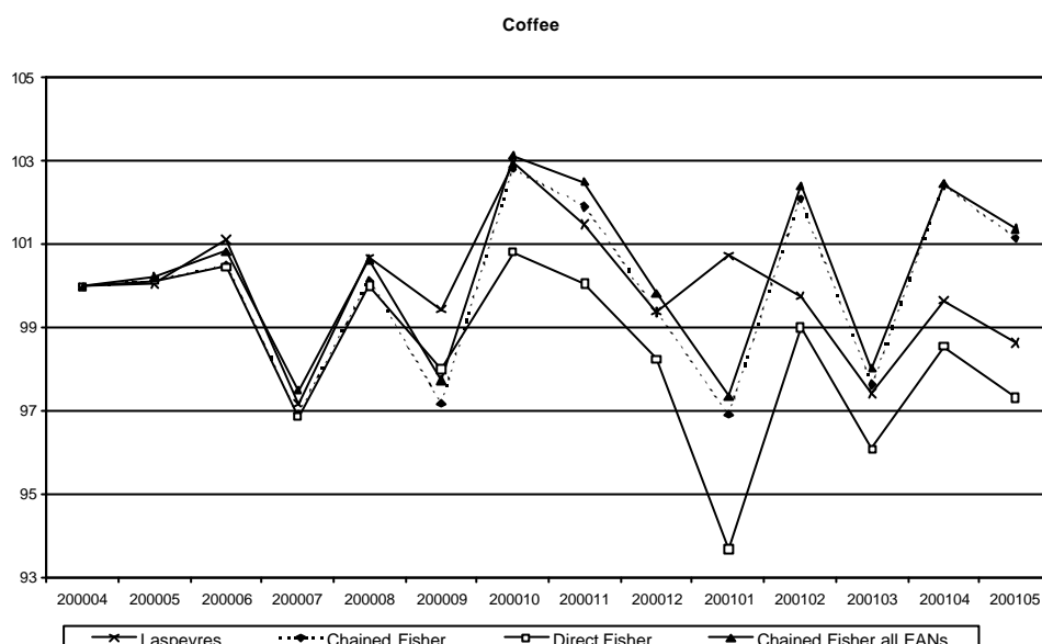
Figure 3: Different indices for the commodity group coffee
