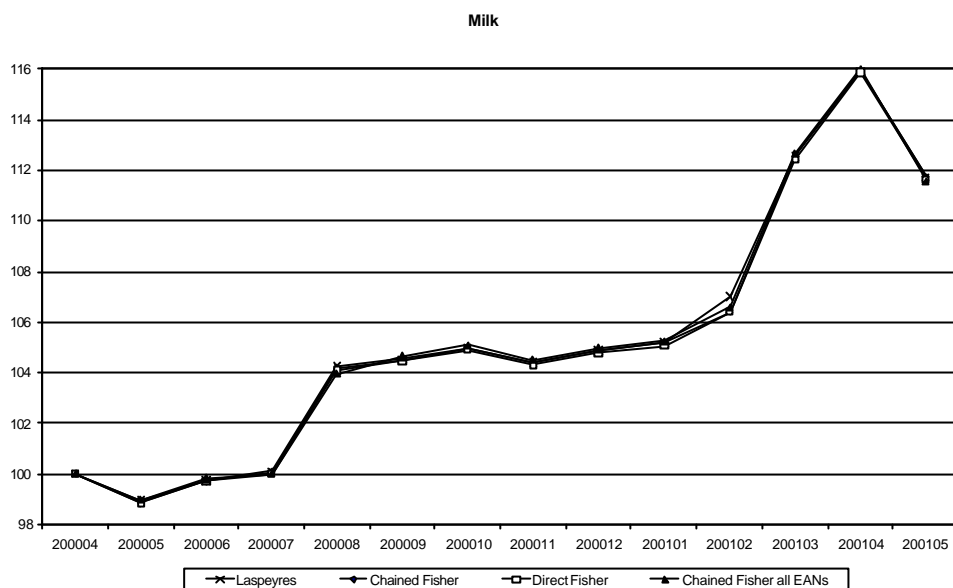
Figure 2: Different indices for the commodity group milk
