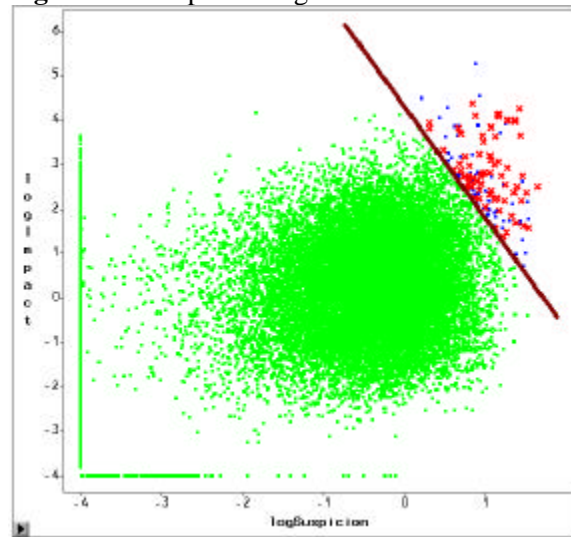
Figure 1 Acceptance region
