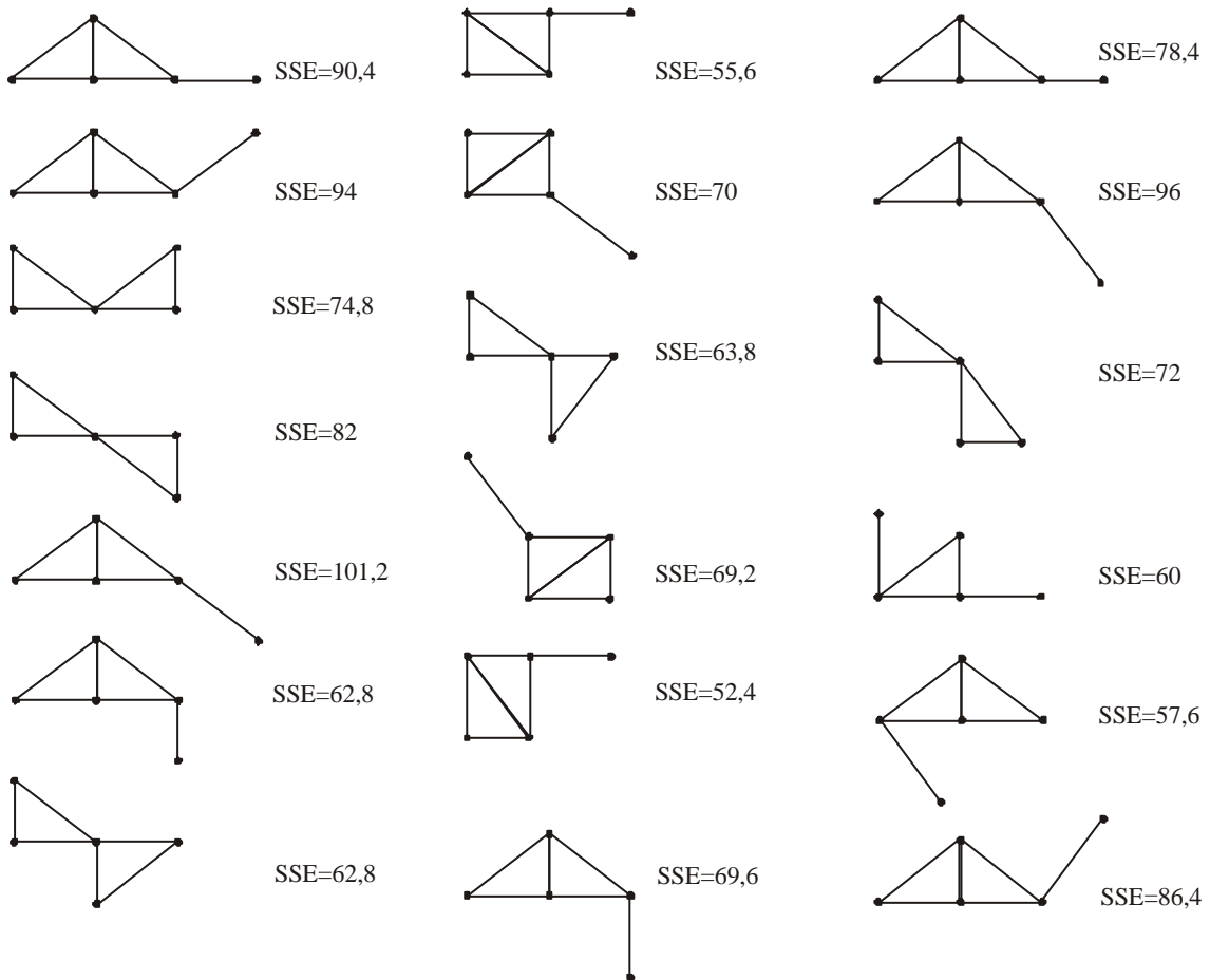
Figure 4. Clusters of 5 points
