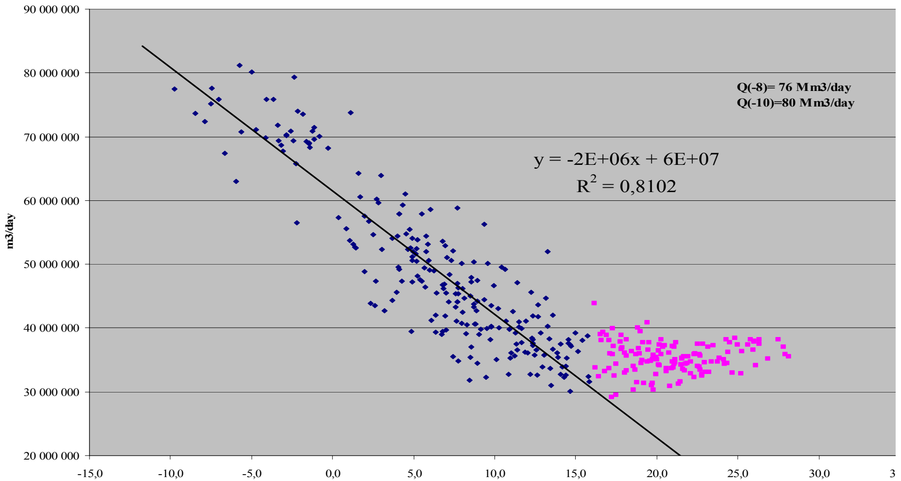
Gas consumption temperature dependency 2002 Hungary
