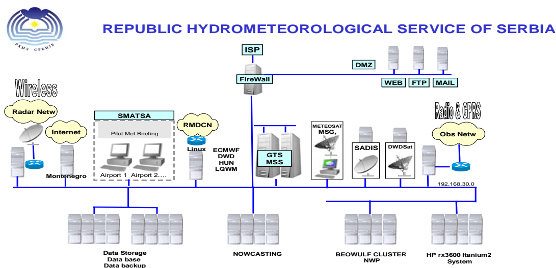
Figure 1: Meteorological telecommunication infrastructure of the Republic Hydrometeorological Service of Serbia ( www.hidmet.sr.gov.yu )
