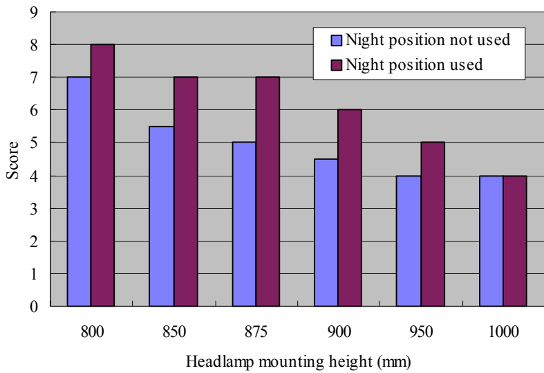
Figure 4 Glare from Following Vehicle (Distance between Vehicles: 5m)
