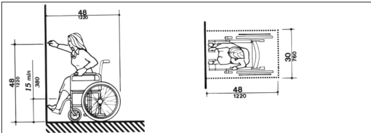
Exhibit 14.6.1 Forward reach from a wheelchair.
