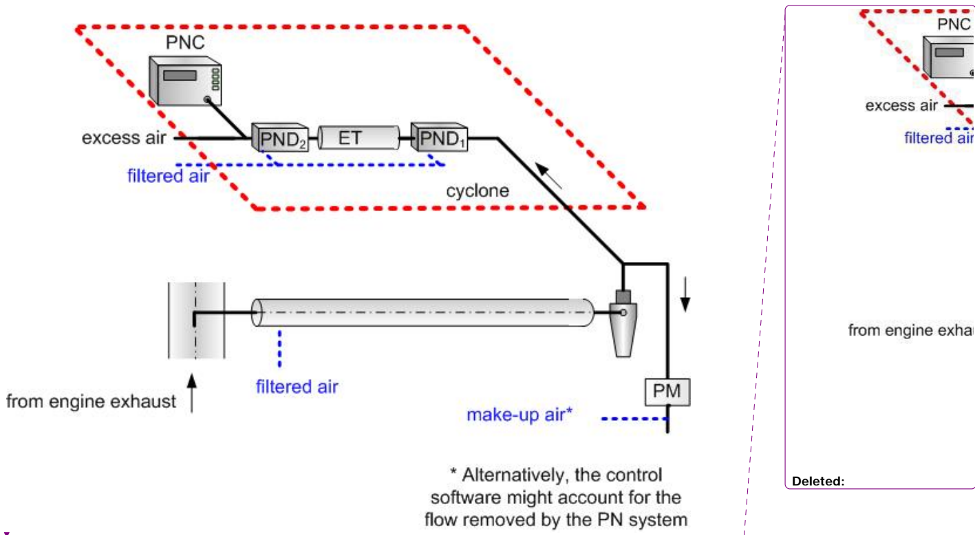
Figure 14: Schematic of Recommended Particle Sampling System – Partial Flow Sampling
