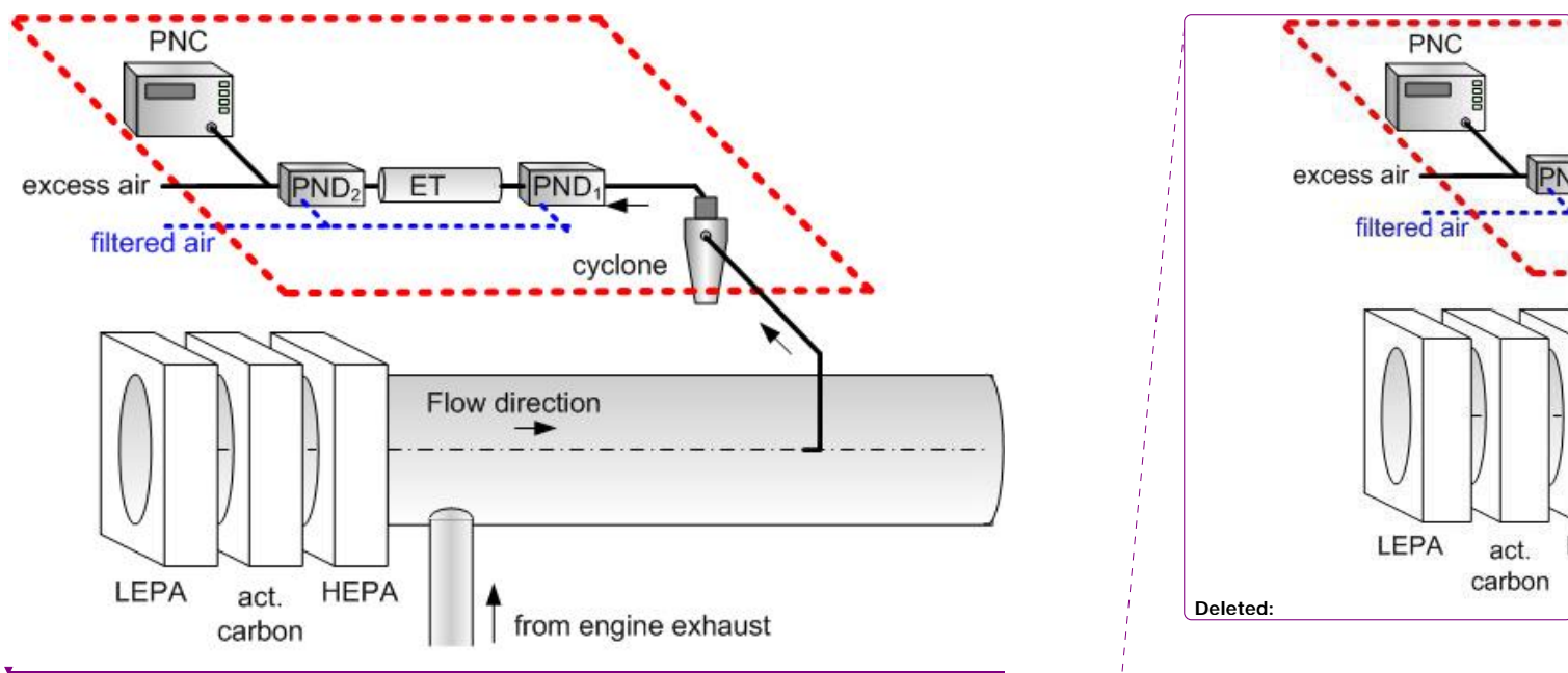
Figure 15: Schematic of Recommended Particle Sampling System – Full Flow Sampling
