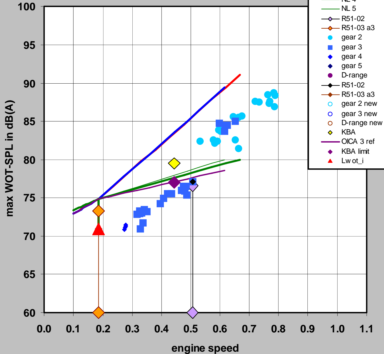
sound emissions R51-ASEP database
