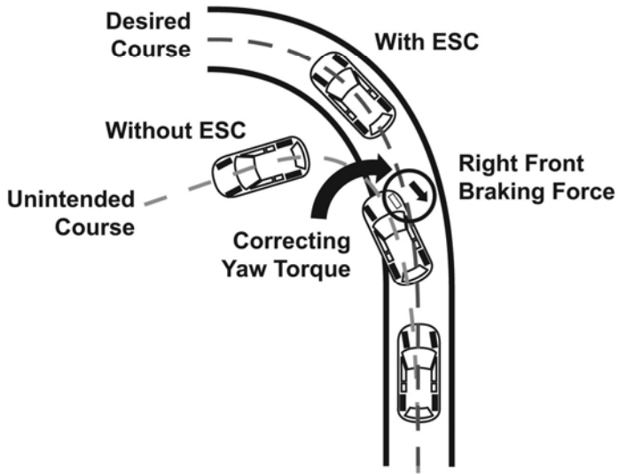
Oversteering ("spinning out")
