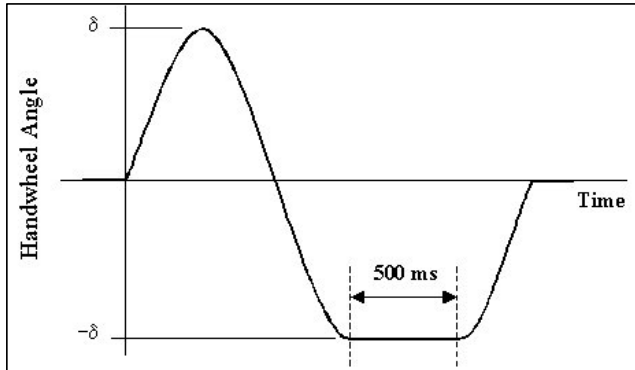
Figure 2. Sine with Dwell steering profile.
