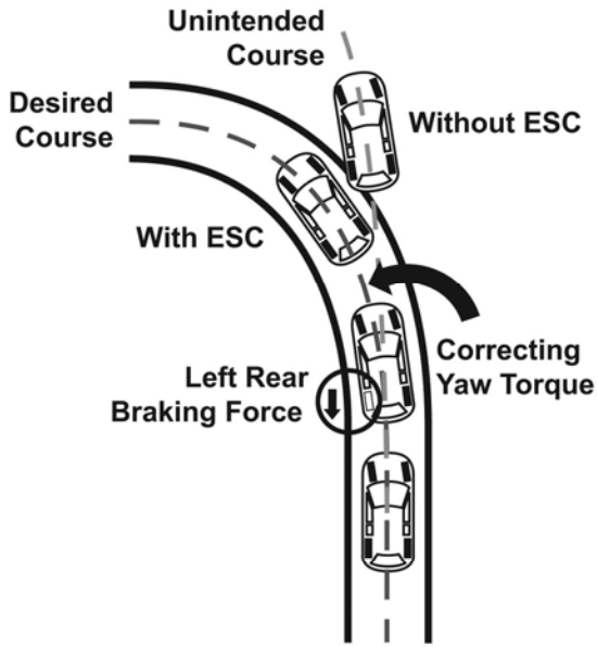
Understeering ("plowing out")
