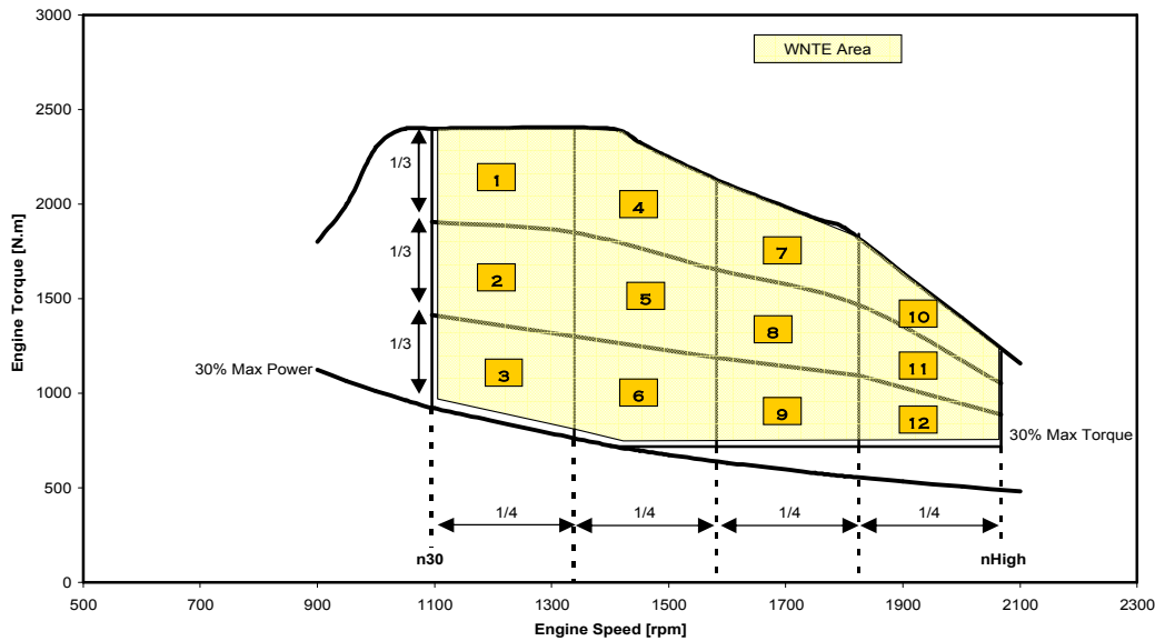
Figure 5: WNTE test cycle grids [new figure to be provided by EC]
