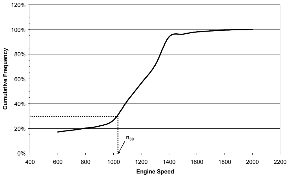
| Figure 3: Example of WHTC cumulative speed frequency distribution
