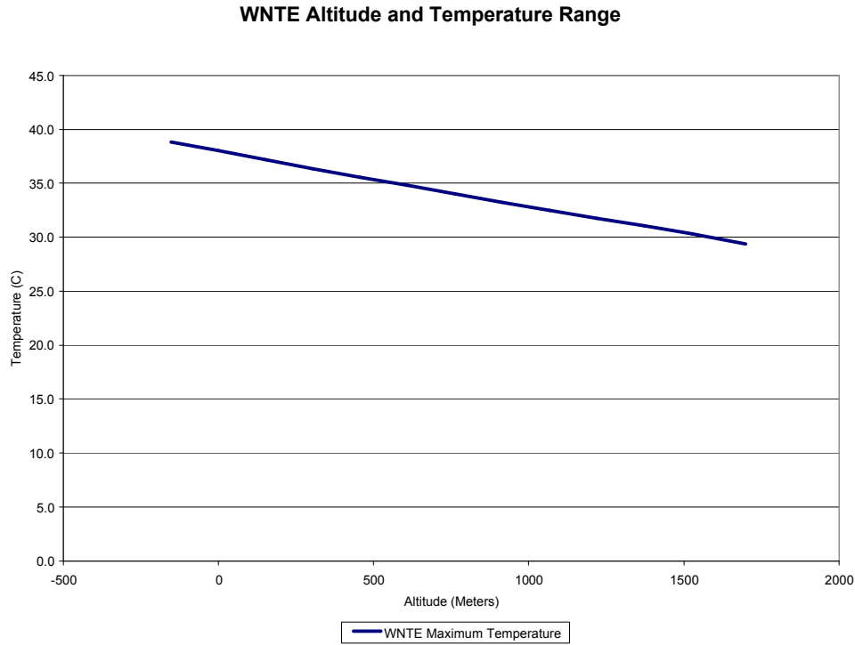
Figure 1 : Illustration of Ambient Altitude and Temperature Conditions
