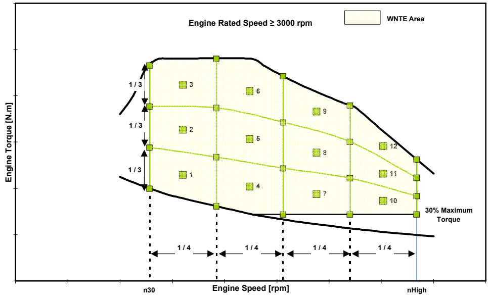
Figure 5: WNTe test cycle grids [new figure to be provided by EC]
