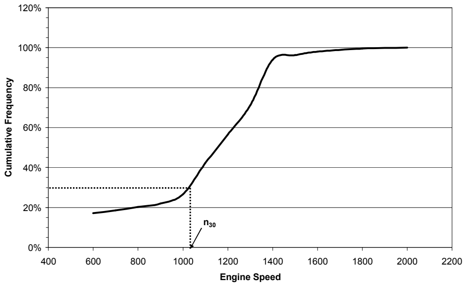
Figure 3: Example of WNTe cumulative speed frequency distribution
