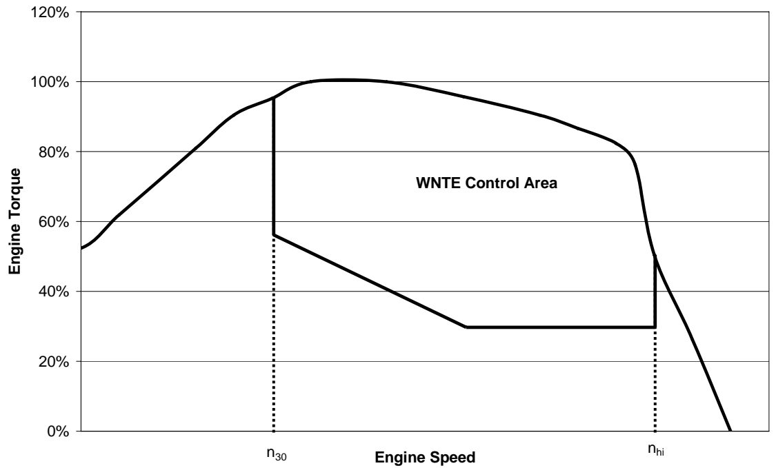
Figure 3: Example Not-To-Exceed Control Area When C Speed > 2,400 rpm
