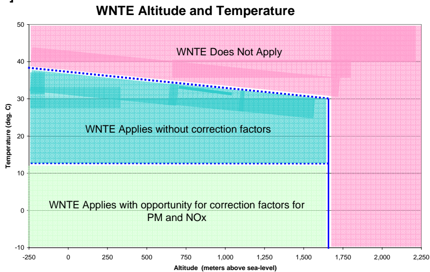
Figure 1 : Illustration of Ambient Altitude and Temperature Conditions [figure to be revised by EPA]
