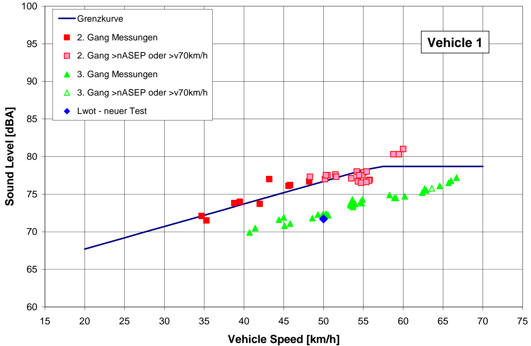
Example - Sound Level versus Vehicle Speed
