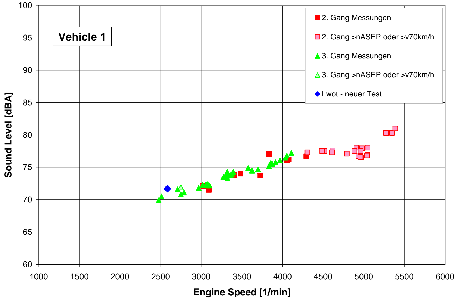
Example - Sound Level versus Engine Speed
