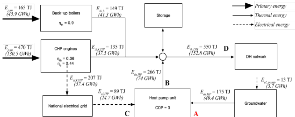
Figure 2 Simplified scheme and energy fluxes of “Canavese” plant*
