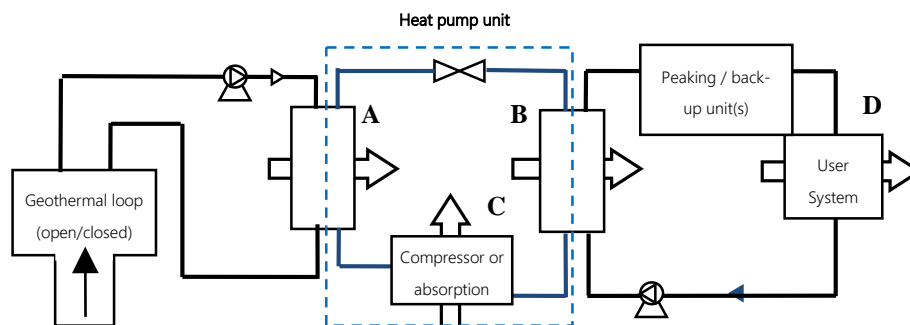
Figure 1 Points of reference for the assessment of GSHP projects in heating mode
