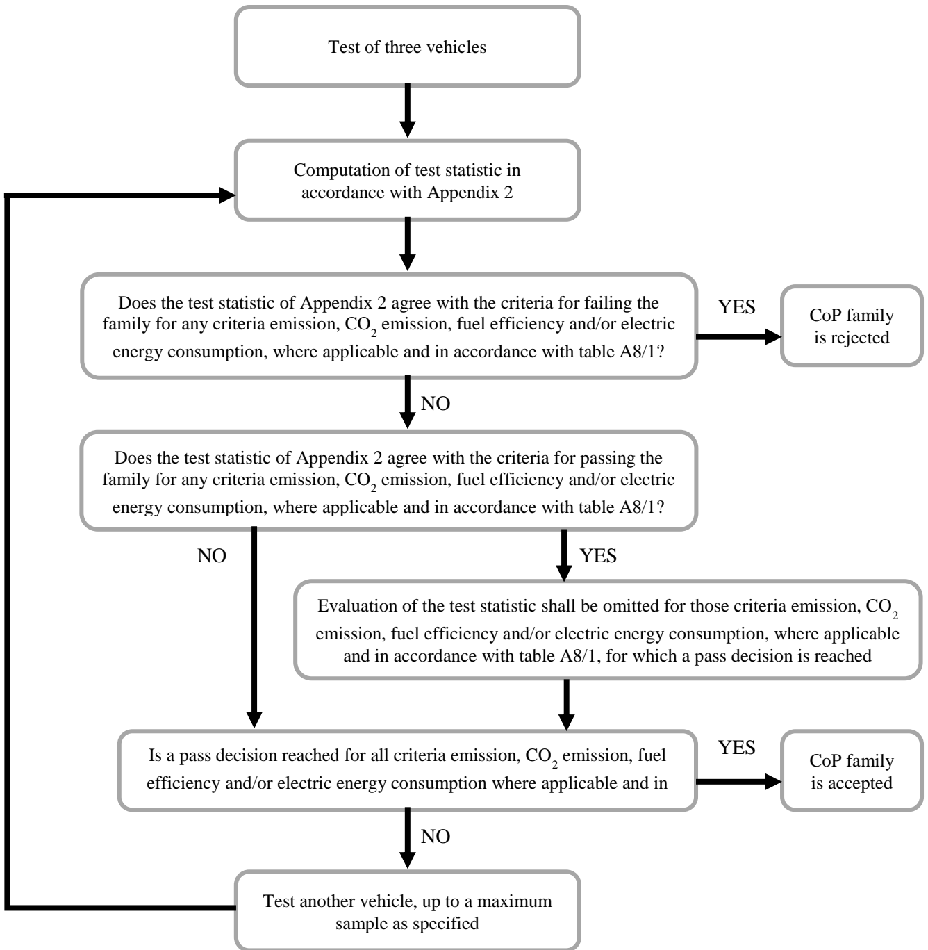
Figure 8/1 Flowchart of the CoP test procedure for the Type 1 test
