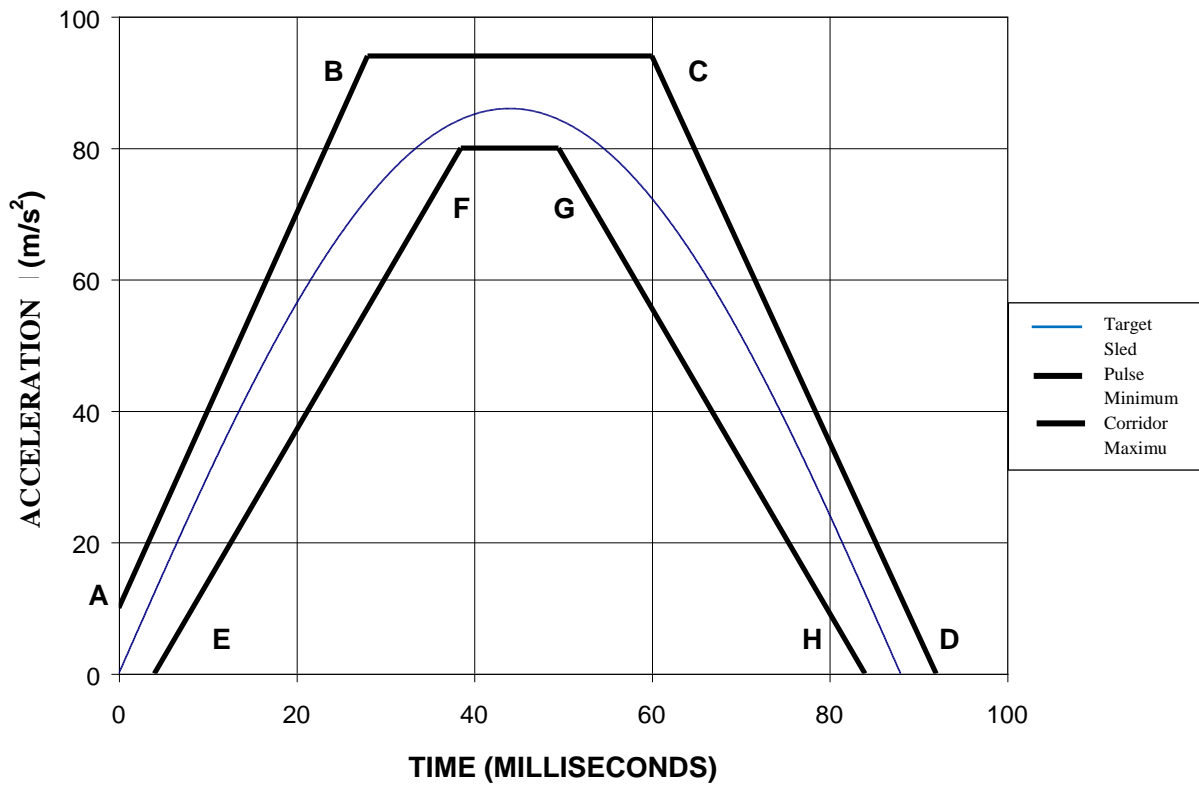
Figure 9-1 8-3 Sled pulse acceleration corridor
