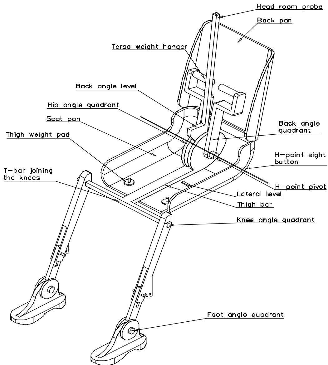
Figure 41-112-1 3-D H machine elements designation
