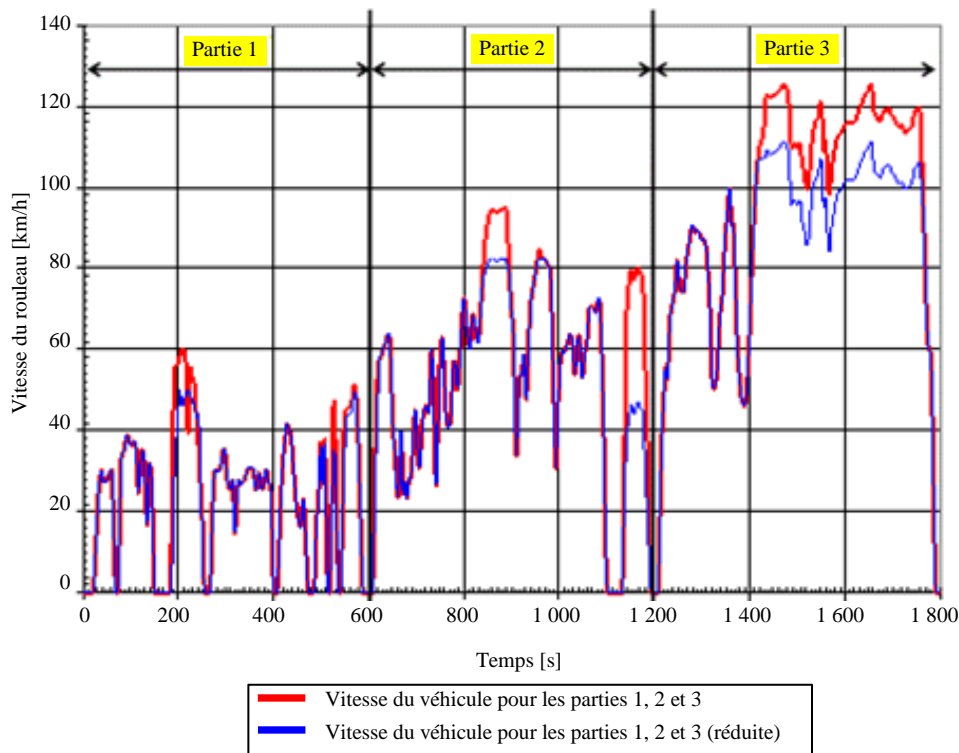
Figure A4.App12/1 Cycle d'essais WMTC
