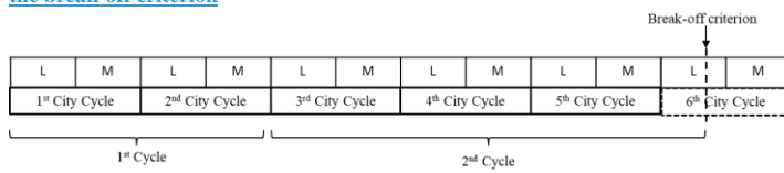
Figure A7/4 Example with an odd number of completed city test cycles before the city cycle with the break-off criterion.
