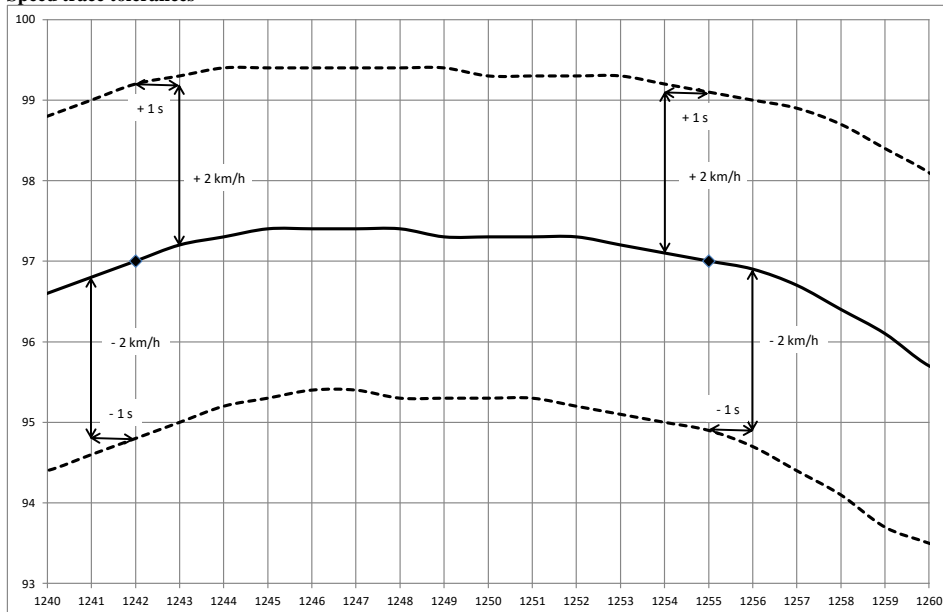
Figure A6/6 Speed trace tolerances
