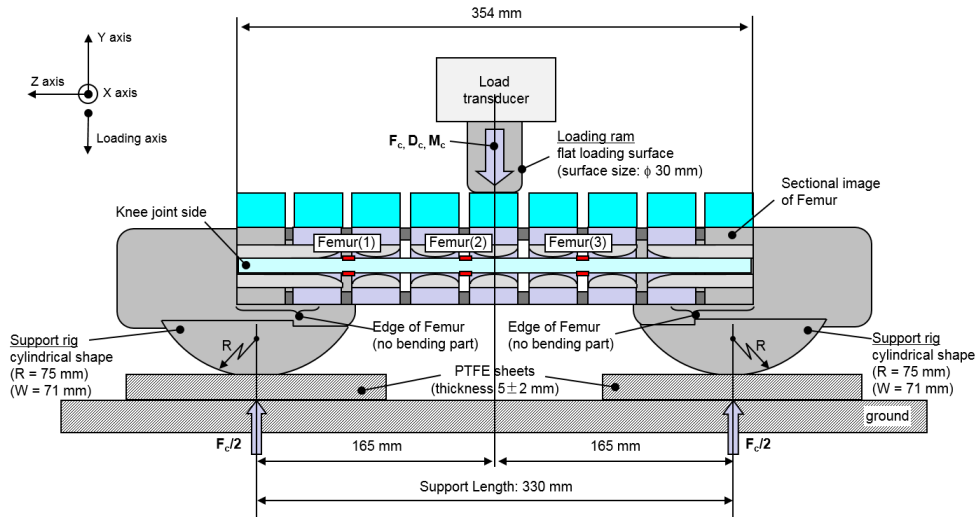
Figure 24 Flexible lower legform impactor: Test set-up for the femur in the static certification test (see paragraph 8.1.1.4.)
