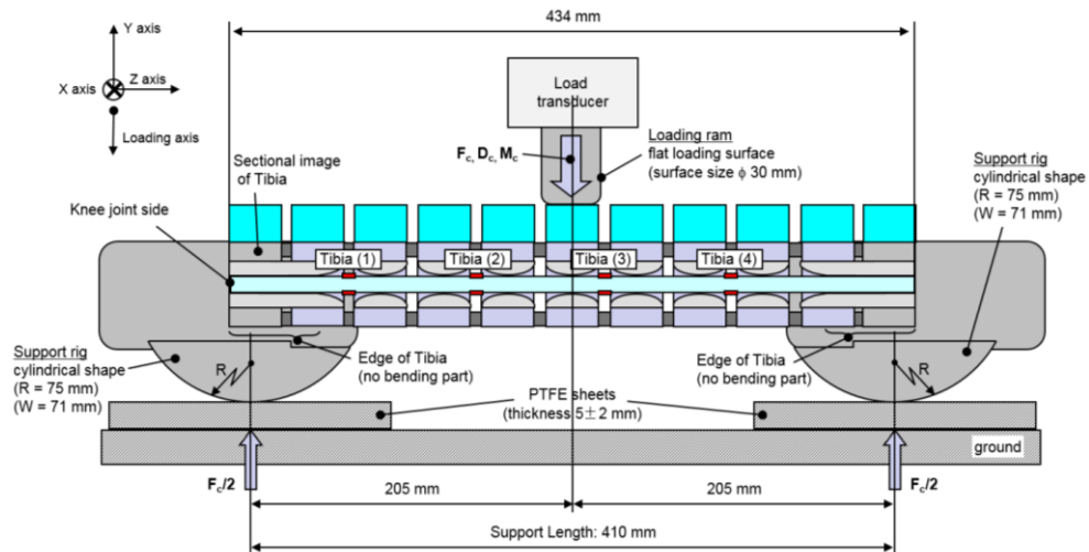
Figure 25 Flexible lower legform impactor: Test set-up for the tibia in the static certification test (see paragraph 8.1.1.4.)
